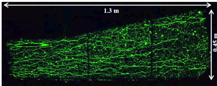
FIGURE 2: Fluorescent impregnated concrete beam seen under ultra-violet light. Experiment VV4. From [6].
