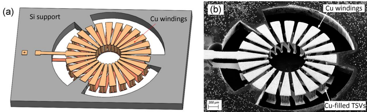
Figure 1: 3D Illustration of air-core toroidal inductor chip (a), and SEM micrograph of fabricated air-core inductor (b).
