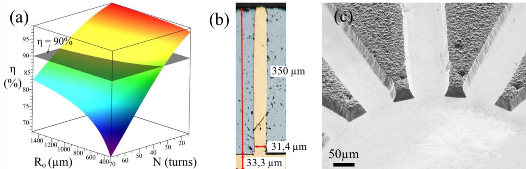
Figure 2: 3D plot of calculated efficiency as a function of number of turns ( N ) and outer radius ( R_o ) (a), (b) 30-μm-diameter, 350-μm-tall Cu-filled TSV, (c) wet-etched copper windings.
