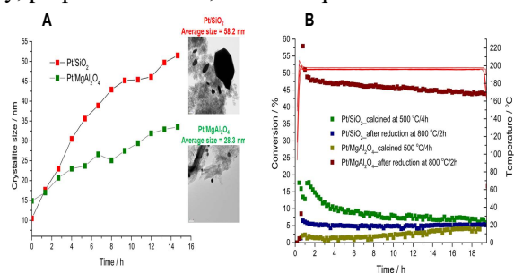
Figure 1 – A: Crystallite size of Pt on different supports (SiO 2 , MgAl 2 O 4 ) determined through in situ XRD measurements and acquired at 750 °C with 10 % O 2 balanced in N 2 during a 15 h period. B: Stability at 200 °C of the Pt/SiO 2 and Pt/MgAl 2 O 4 catalyst for propene oxidation reaction, before and after a reduction pretreatment at 800 °C in 5 % H 2 balanced in N 2 for 2 h.
