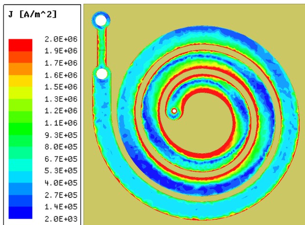
Fig.6. The current density at 10 MHz (top view)
