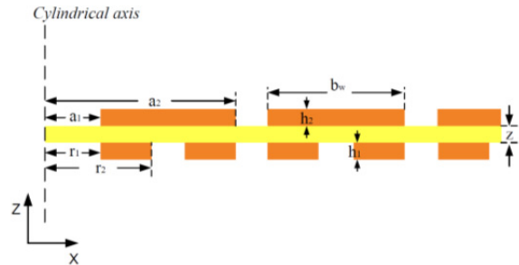
Fig. 4. A generic cross-section of a PCB inductor
