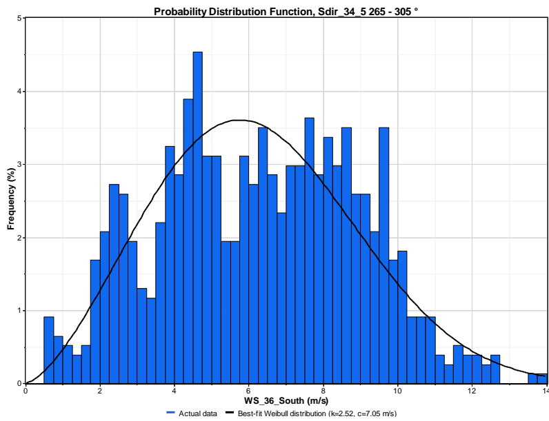
Figure 28 Speed frequencies
