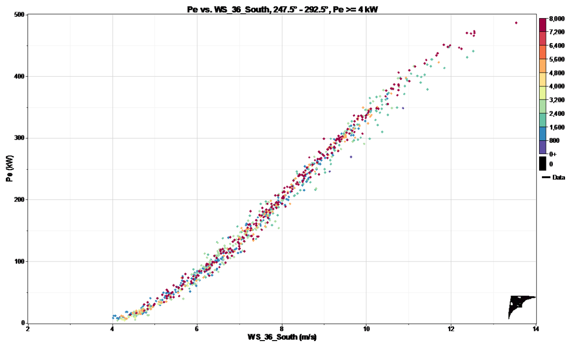
Figure 32 Generated Power
