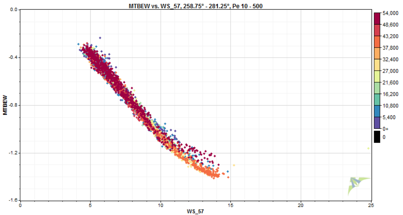
Figure 12 Example of no drift. 10 min averages of tower bottom bending moment East West direction vs wind speed (top cup anemometer at 57m) color coded by time
