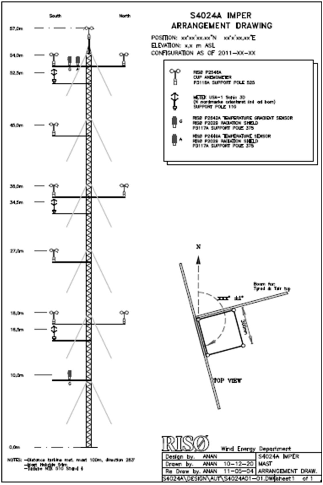
Figure 3 Tall mast
