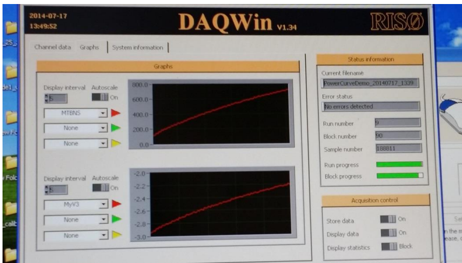
Figure 17 Screenshot of DAQwin Software during continuous pull. The first graph shows the applied load in Kg and below the correspctive output from the strain gauge in Volt, both over time.
