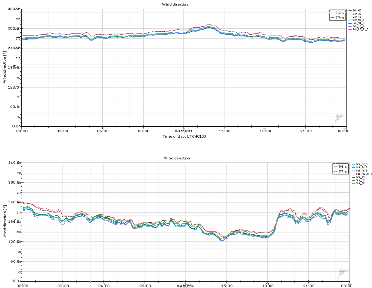
Figure 25 Comparison of all mast wind directions measurements existing at R Risø campus. G reen-V27 mast direction measurements in green scale, Nordtank tall mast in blue scale, s Small mast in purple (no data) while the Risø Tower wind vanes measurements are in legend without the “Sdir” prefix during the 17 (upper) and 22 of March (lower) 2014, two recent days where the wind has been blowing all day from mast-turbine direction.
