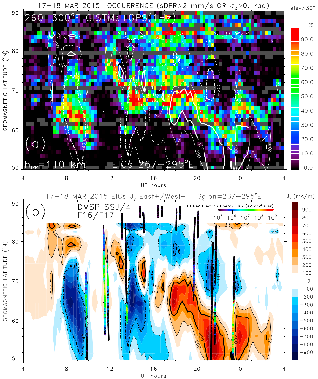
Figure 10. (a) The phase scintillation occurrence of \sigma_{\phi} > 0.1 \text{ rad} or \text{sDPR} > 2 \text{ mm/s} as a function of AAGCM latitude and UT for CHAIN combined with 1 Hz GPS receivers for data from 04:00 UT on 17 March to 03:59 UT on 18 March 2015. Contour plots of the westward and eastward equivalent ionospheric currents are shown in white broken and solid lines, respectively. (b) Westward and eastward equivalent ionospheric currents are highlighted in blue and brown shades. Superposed are tracks of DMSP F16 and F17 satellites that crossed the longitude sector between 260° and 300°.
