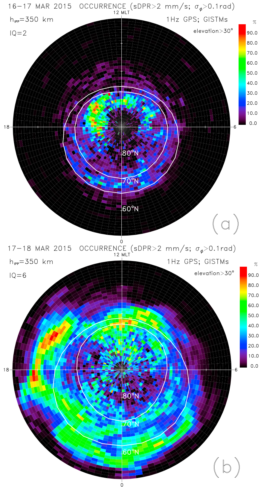
Figure 3. The phase scintillation occurrence of \sigma_{\phi} > 0.1 rad or \sigma_{DP} > 2 mm/s for CHAIN combined with 1 Hz GPS receivers for data from (a) 04:00 UT on 16 March to 03:59 UT on 17 March and (b) 04:00 UT on 17 March to 03:59 UT on 18 March 2015. The scintillation occurrence is mapped in coordinates of AACGM latitude and MLT. Boundaries of the statistical auroral oval are shown.
