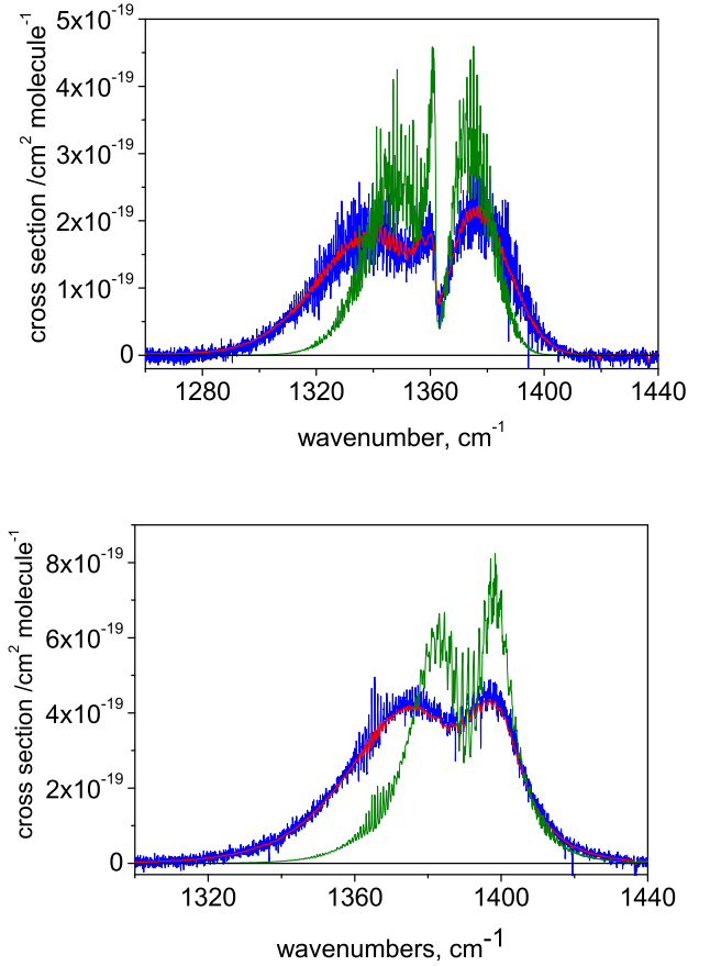
Figure 3. \text{SO}_2 (upper) and \text{SO}_3 (lower) absorption cross-sections at 400 C: 0.09 \text{cm}^{-1} (blue, boxcar), 0.5 \text{cm}^{-1} (red, triangular). Cross-section from PNNL data base at 25 C (olive, 0.112 \text{cm}^{-1} , boxcar) are shown for comparison.
