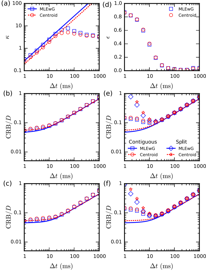
FIG. 8. Cramér-Rao bound (CRB) on the standard error of any unbiased estimator of the diffusion coefficient as function of time lapse \Delta t for a time series of limited recording time t_{\text{tot}} = (N + 1)\Delta t . Lines mark theoretical results [from Eqs. (17) and (19)]; symbols mark numerical results (Appendix A); error bars are smaller than symbol sizes. (a) Signal-to-noise ratio, \kappa , in a single frame as function of \Delta t . (b, c) CRB as function of \Delta t when all N + 1 positions are found: (b) for unknown \sigma , (c) for independently determined \sigma . (d) Probability \epsilon for localization to fail as function of \Delta t . (e, f) CRB as function of \Delta t when the particle is only localized in a fraction 1 - \epsilon of the N + 1 images recorded, for the two different scenarios discussed in the main text: (i) where a contiguous trajectory can be constructed from the found positions (contiguous), or (ii) where the particle cannot be reidentified after a position is missing and the trajectory is split into smaller time series (split), (e) for unknown \sigma , (f) for known \sigma . In all panels the total recording time is t_{\text{tot}} = 10 s, the rate of photon emission of the fluorescent particle is r = 10 kHz, the width of the stationary PSF is s_a = 153 nm, the background-to-signal ratio in images is q = 1 , the shutter is held continuously open ( R = 1/6 ), and the particle undergoes 2D diffusion with diffusion coefficient D = 1 \mu\text{m}^2\text{s}^{-1} .
