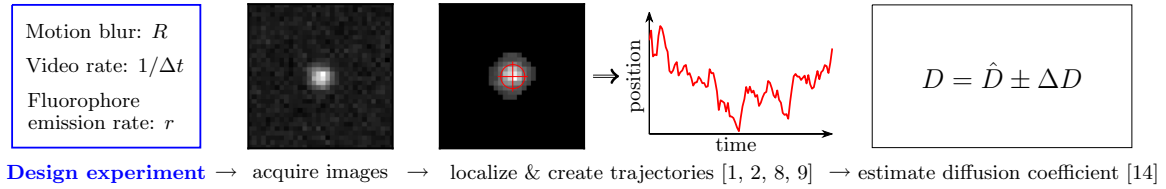
FIG. 1. Workflow for estimating diffusion coefficients from camera-based single-particle-tracking experiments. We are here concerned with optimizing the first step: how to choose experimental parameters (motion blur, video rate, and photon emission rate of the tracked fluorophore) for optimal precision of estimates of the diffusion coefficient of a tracked particle. The motion blur is characterized by a motion blur coefficient , R \in (0, 1/4) [Eq. (8)] [11]. The motion blur coefficient, R , and video rate, given by 1/\Delta t , where \Delta t is the time lapse between measurements, may normally be controlled directly; the photon emission rate of the fluorophore, r , may be controlled indirectly, e.g., by varying the laser intensity or by the choice of fluorophore itself. Optimization of other steps in the workflow is addressed in the references given in the legends.
