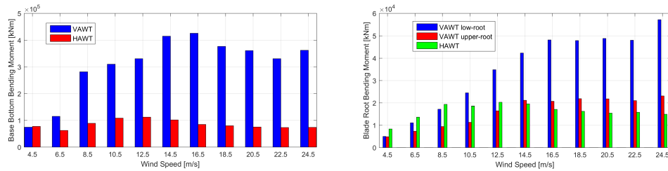
Fig. 3. Extrapolated 50 year return period extreme values of turbine base bottom bending moment (left) and blade root bending moment (right) as a function of wind speed for vertical and horizontal axis wind turbines under normal power production.
