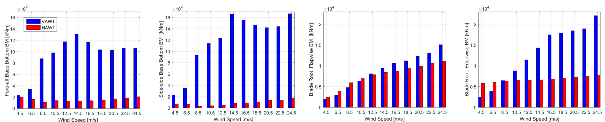
Fig. 4. Equivalent 1 Hz fatigue base bottom bending moments as a function of wind speed (first and second subplots) and equivalent 1 Hz fatigue blade root bending moments (third and fourth subplots) under normal power production.
