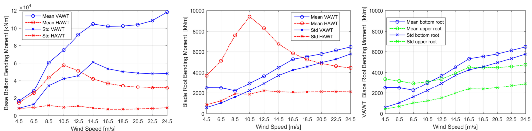
Fig. 2. Turbine base bottom bending moment (left) and blade root (low root for VAWT) bending moment (middle) as a function of wind speed for vertical and horizontal axis wind turbines. Right: Blade upper and low root bending moments as a function of wind speed for the VAWT.
