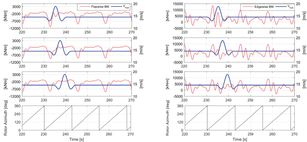
Fig. 7. Time series of VAWT blade-1 low root bending moments M_x (left subplots) and M_y (right subplots) during the EOG event at 14.5 \text{ m/s} . The gust frontal passage passes the rotor plane at 3 different time stamps (corresponding to different rotor orientations), each one represented at the 1 st , 2 nd and 3 rd row of subplots.
