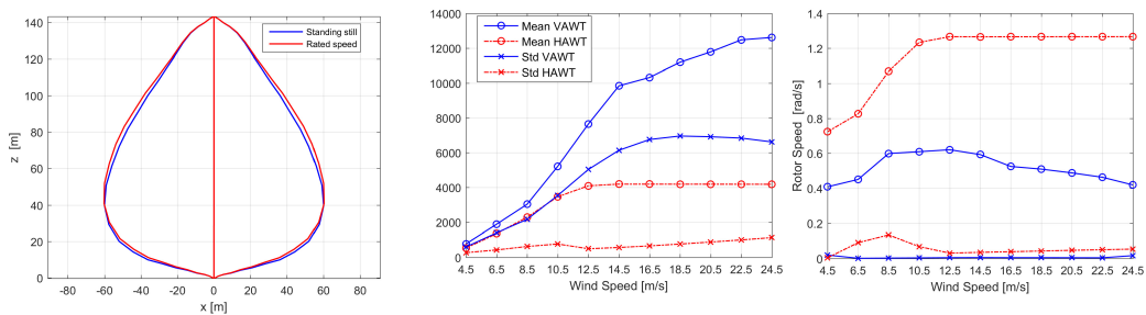
Fig. 1. VAWT rotor centreline at standing still and rated rotor speed (left). Rotor torque (centre) and rotor speed (right) as a function of wind speed for vertical and horizontal axis wind turbines.
