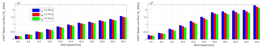
Fig. 6. Influence of turbulence intensity in the equivalent 1 Hz fatigue VAWT blade low root bending moments under normal power production.
