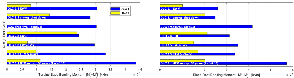
Fig. 11. Comparison of the VAWT DLCs absolute maximum bending moments at the turbine base (left) and the blade root section (right).
