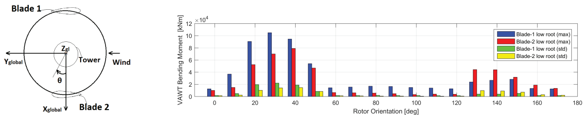
Fig. 9. Parked and locked VAWT rotor at different orientations exerted to 50 year recurrence period extreme winds. Left: Rotor cross-section at equator height, depicting the orientation of the blades. Right: Maximum and standard deviation of blade 1 and 2 low root bending moments.
