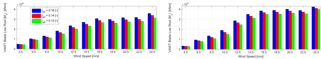
Fig. 5. Influence of turbulence intensity in the extrapolated 50 year return period extreme VAWT blade low root bending moments under normal power production.
