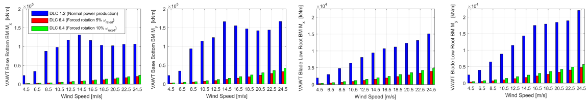
Fig. 10. VAWT equivalent 1 Hz fatigue base bottom bending moments M_x and M_y as a function of wind speed (first and second subplots) and equivalent 1 Hz fatigue blade root bending moments M_x and M_y (third and fourth subplots) comparison of DLC 1.2 and DLC 6.4.
