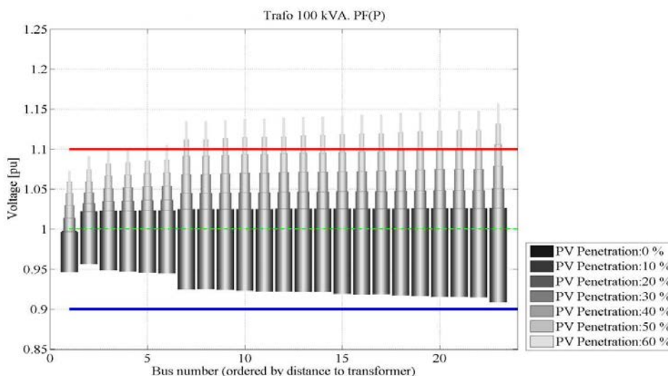
Figure 23. Maximum voltages at different levels of PV penetration along feeder 1 via PF(P).
