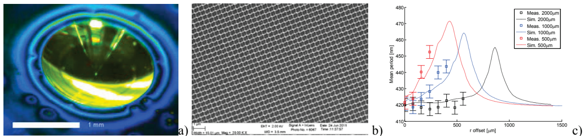
FIGURE 3. a) The deformed nickel after embossing, b) characterization of the nanostructured surface of the aluminum tool inserts with SEM, c) comparison of measured and numerically calculated periods of the nanostructure in the three different test cases.
