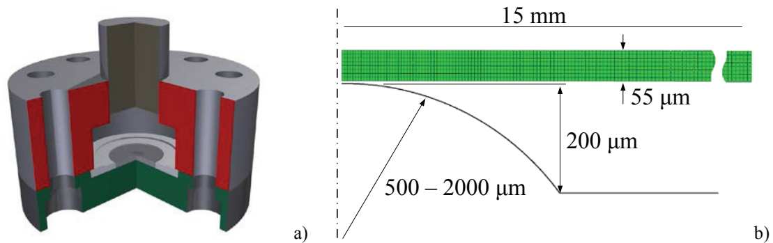
FIGURE 2. a) The device for high pressure nanoimprinting of the nickel foil into the aluminium curved surface, b) Geometry and mesh of the 2-D axisymmetric numerical model
