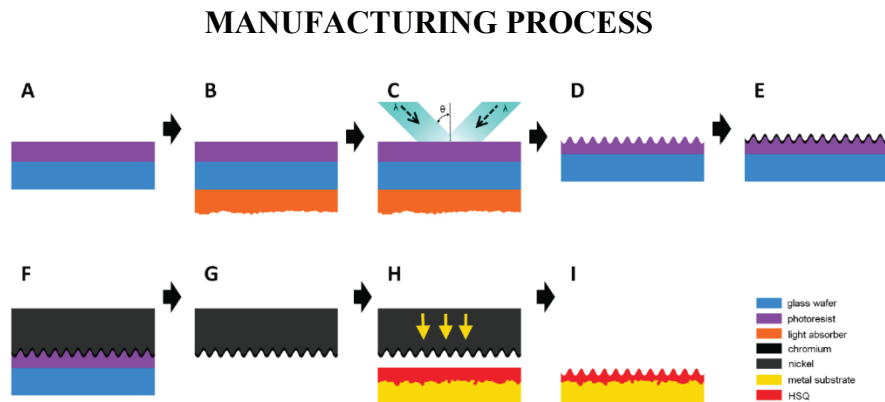
FIGURE 1. Schematic illustration of the manufacturing process, from preparation of the 426 nm pattern on the wafer (A-D), to electroforming the flexible nickel foil (E-G), further on to nanoimprint lithography into a material called HSQ on top of the final metal substrate (H-I).
