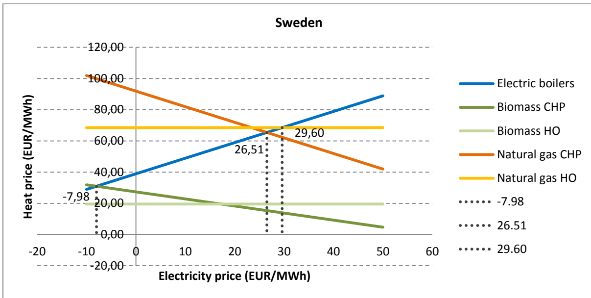
Figure 3 Sweden: Short term marginal cost of heat as a function of electricity price. The blue line indicates the cost of electric boilers. The electricity prices at which the marginal heat cost of electric boilers are equal to that of natural gas HO and CHP, and biomass CHP are all marked with a dashed line.
