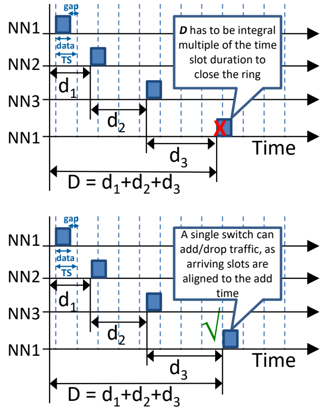
Fig. 2. A ring network with length that is not (top) and that is (bottom) an integer multiple of the time slot duration
