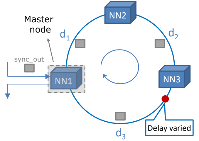
Fig. 4. Overview of the implemented synchronization plane
