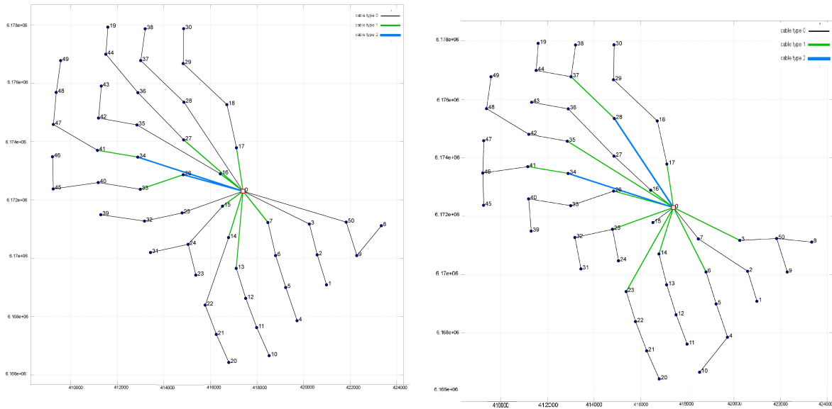
Figure 9 Optimized layouts for HR3 with maximum 18 connections to the substation: plot on the left is the optimal layout considering only CAPEX costs while on the right is the layout optimized considering cable losses over 25 years. Black cables represent cable type 1, green are cable type 2 and blue are cable type 2 overloaded.
