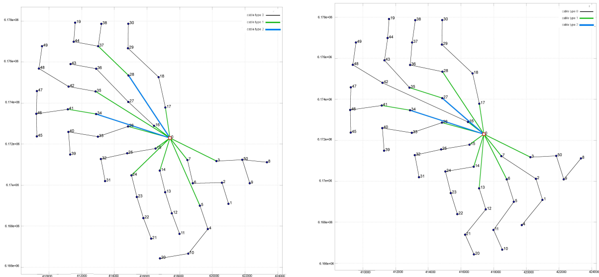
Figure 8 Optimized layouts for HR3: On the left is the optimal layout considering cable losses over 25 years, while on the right is the layout optimized by considering only CAPEX costs. Black cables are of cable type 1, green are of cable type 2, and blue are of cable type 2 carrying 5 turbines.
