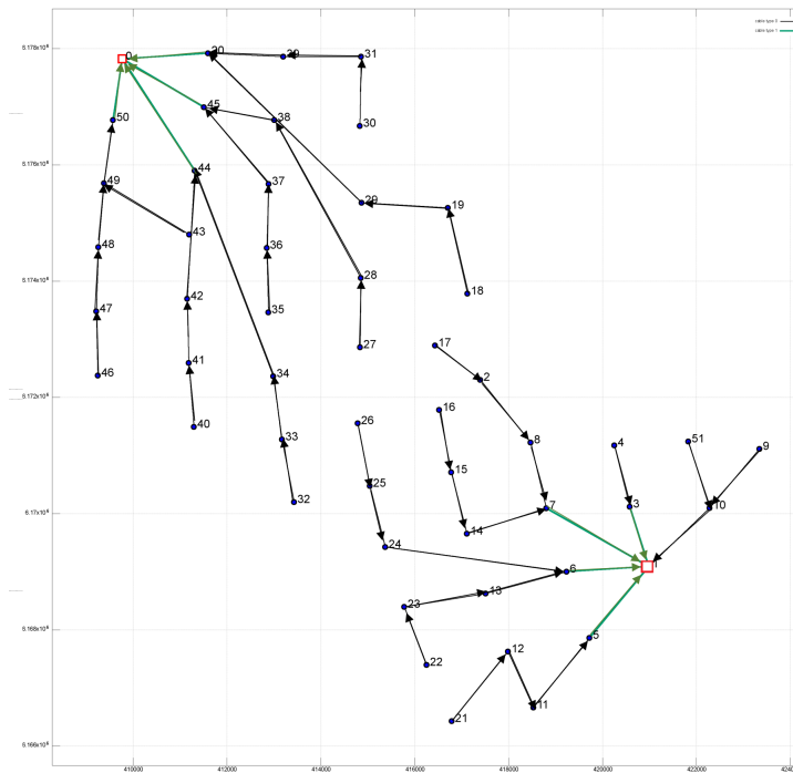
Figure 2 A feasible cable routing; arcs are directed according to the electric current flow, i.e., towards roots (substations).
