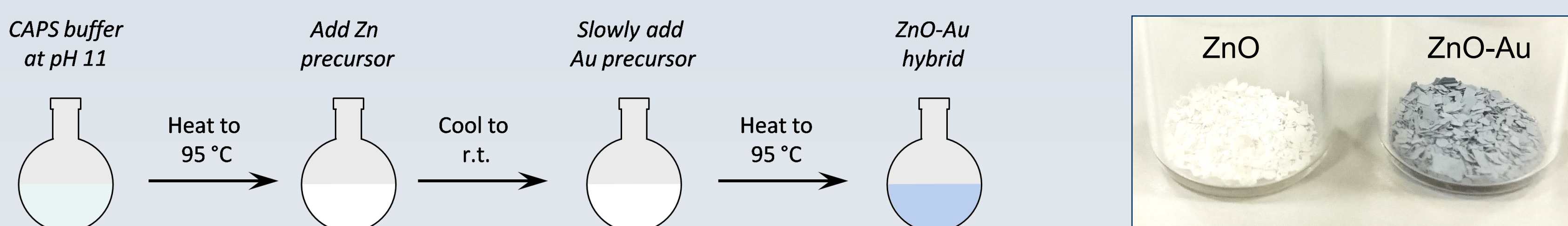
Scheme 1. Synthesis of ZnO and ZnO-Au hybrids. N -cyclohexyl-3-aminopropane-sulfonic acid (CAPS) buffer is adjusted to pH 11 and heated to 95 °C before addition of Zn precursor solution. After formation of ZnO, the mixture is cooled and HAuCl 4 is added dropwise. Finally, the mixture is heated again reducing the Au precursor forming ZnO hybrids.
