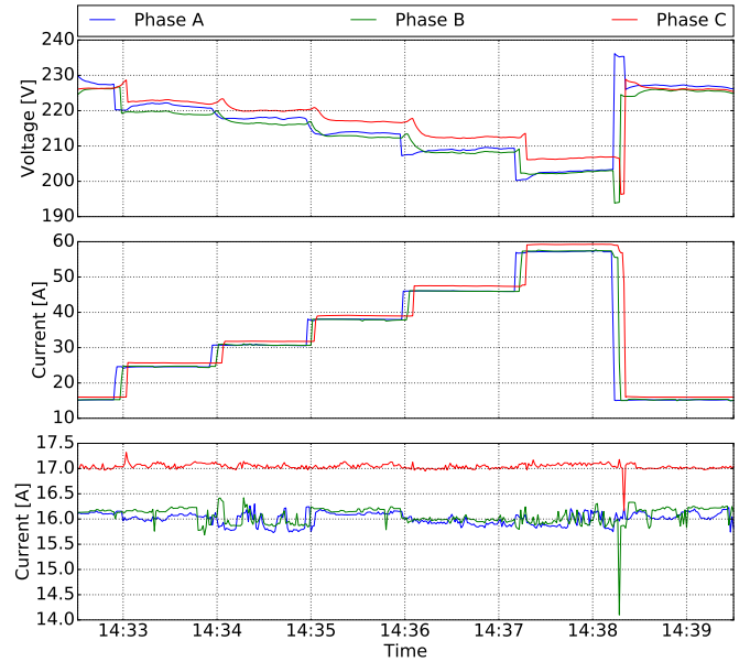
Fig. 5: Voltage and load current measurements for EV uncontrolled charging - test scenario I
