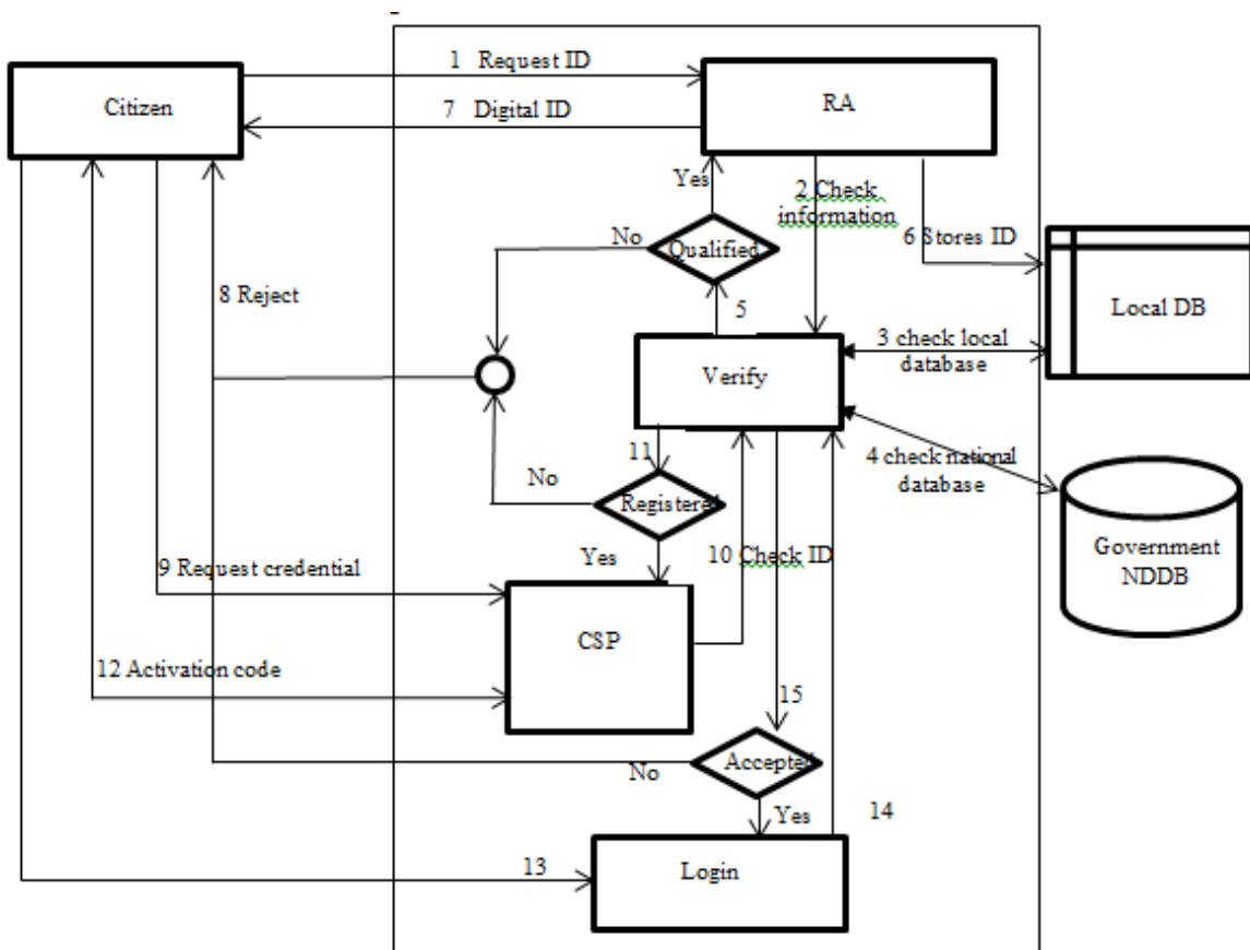
Figure 1A Simple Model of Online Authentication
