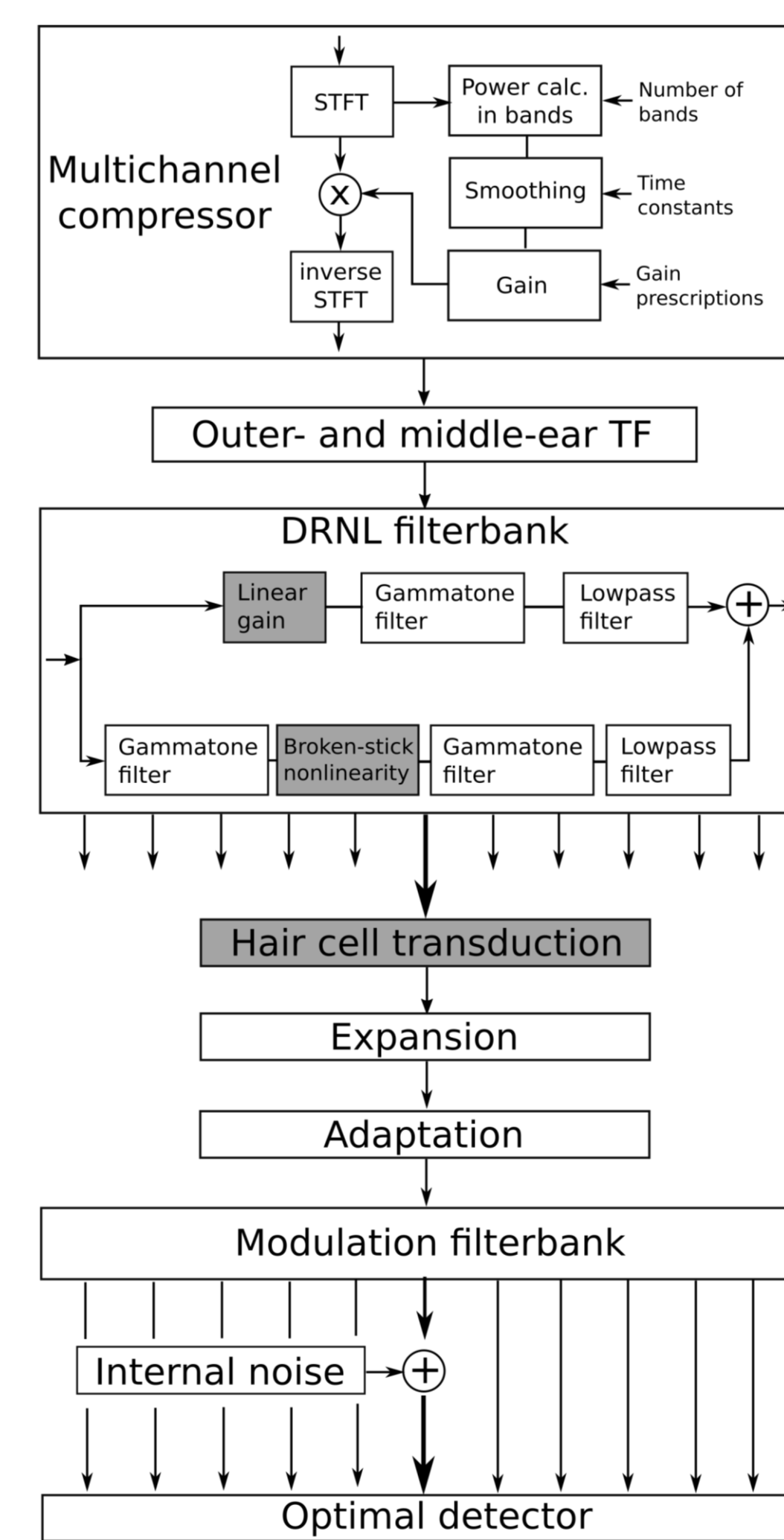
Fig. 3. CASP model structure including the hearing-aid compression preprocessing. Grey-colored blocks represent the model stages subject to changes due to the individual hearing loss.
