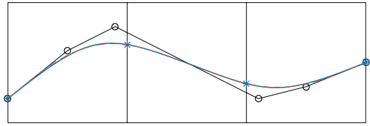
Figure 15. The curvature continuous construction. A single cubic spline curve where the images of the knots are on the block boundaries. In dashed red we have plotted the true elastic curves that have the same length and endpoints as the polynomial pieces. The tangents corresponding to the extreme points of the cubic curve are also prescribed.
