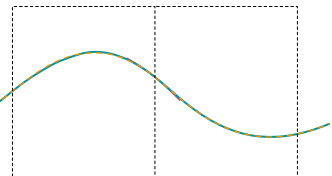
Figure 11. Transitions between elastica.
