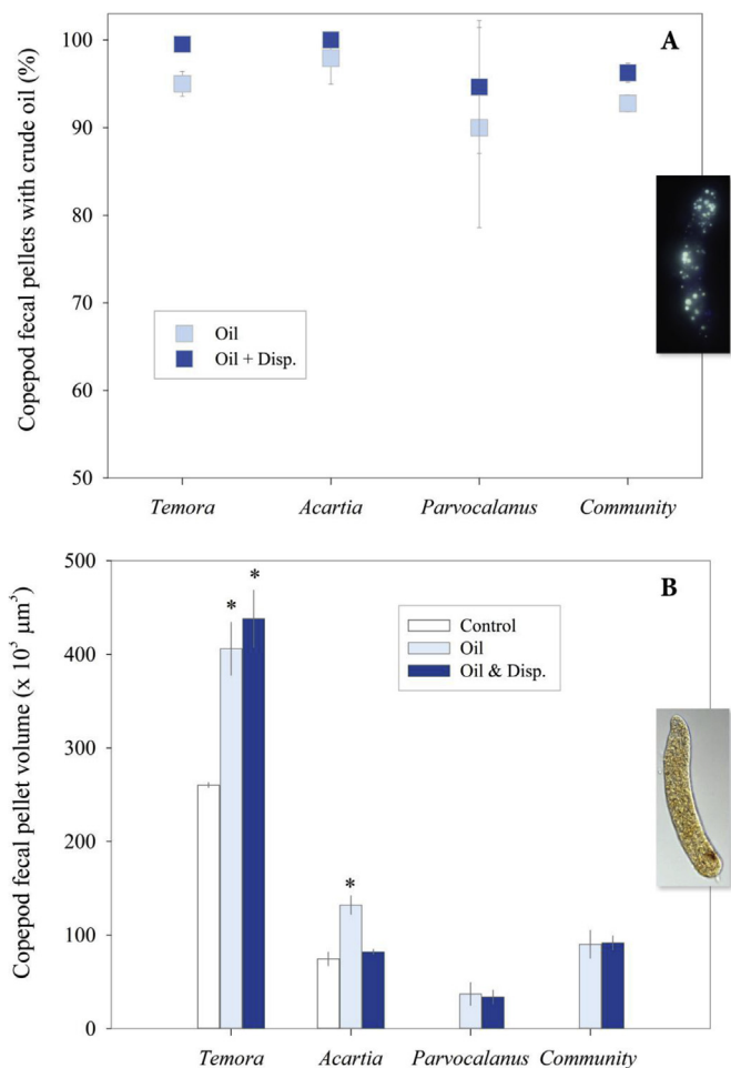
Fig. 2. Percent of fecal pellets containing crude oil droplets (A) and mean fecal pellet volume (B) after exposing copepods Temora turbinata , Acartia tonsa , Parvocalanus crassirostris and natural copepod assemblages (Community) to crude oil (Oil) or dispersant treated oil (Oil + Disp) emulsions. Error bars indicate standard deviation. Note that volume of fecal pellet in control treatments was only determined for A. tonsa and T. turbinata . Asterisk indicates significantly different than the corresponding controls ( p < .05 ).
