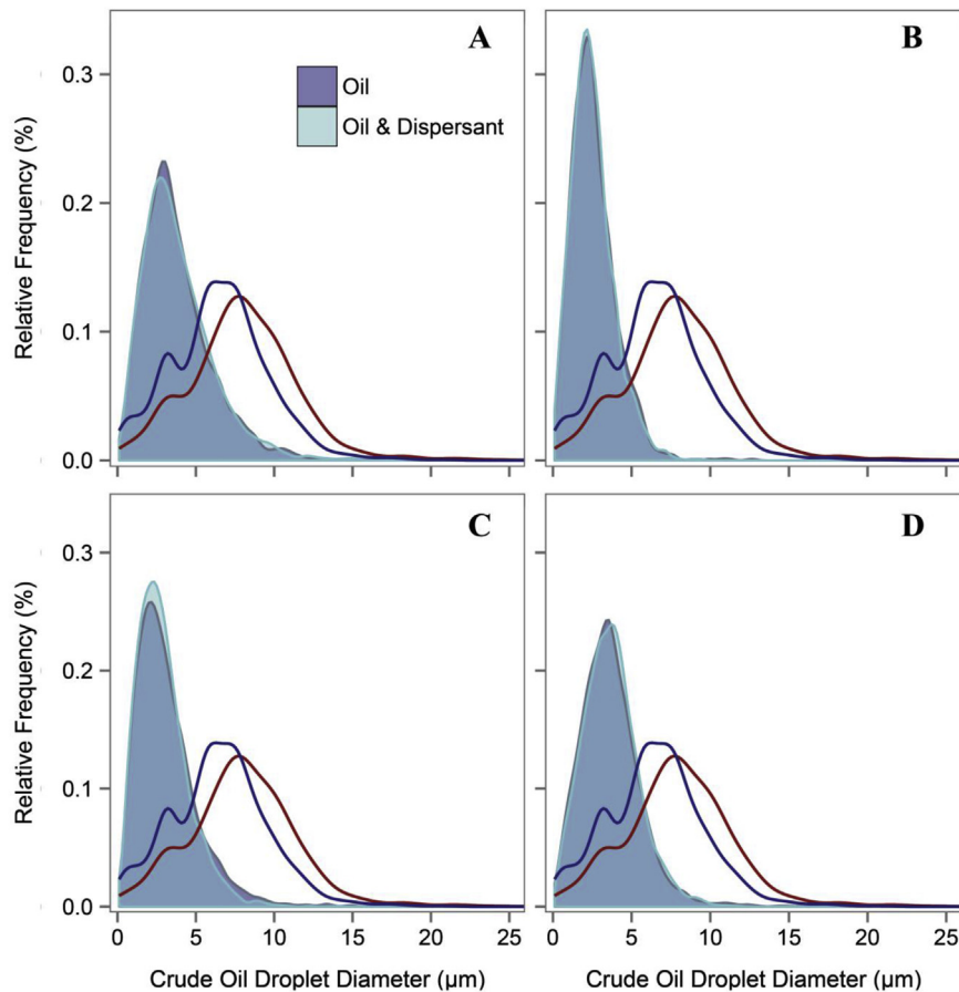
Fig. 3. Relative frequency of crude oil droplet size ingested by copepods and in crude oil emulsions. Diameter of crude oil droplets defecated by Temora turbinata (A), Acartia tonsa (B), Parvocalanus crassirostris (C) and natural copepod assemblages (D) exposed to crude oil (shaded dark blue) or dispersant treated oil (shaded light blue) emulsions. Red and blue lines are the size of droplets in crude oil emulsions added to experimental bottles without dispersants and with dispersants, respectively. In all cases the relative frequency data were fit to a density function using R software. Note that there is an overlap in the diameter of ingested oil droplets between crude oil (shaded dark blue) or dispersant treated oil (shaded light blue) treatments.
