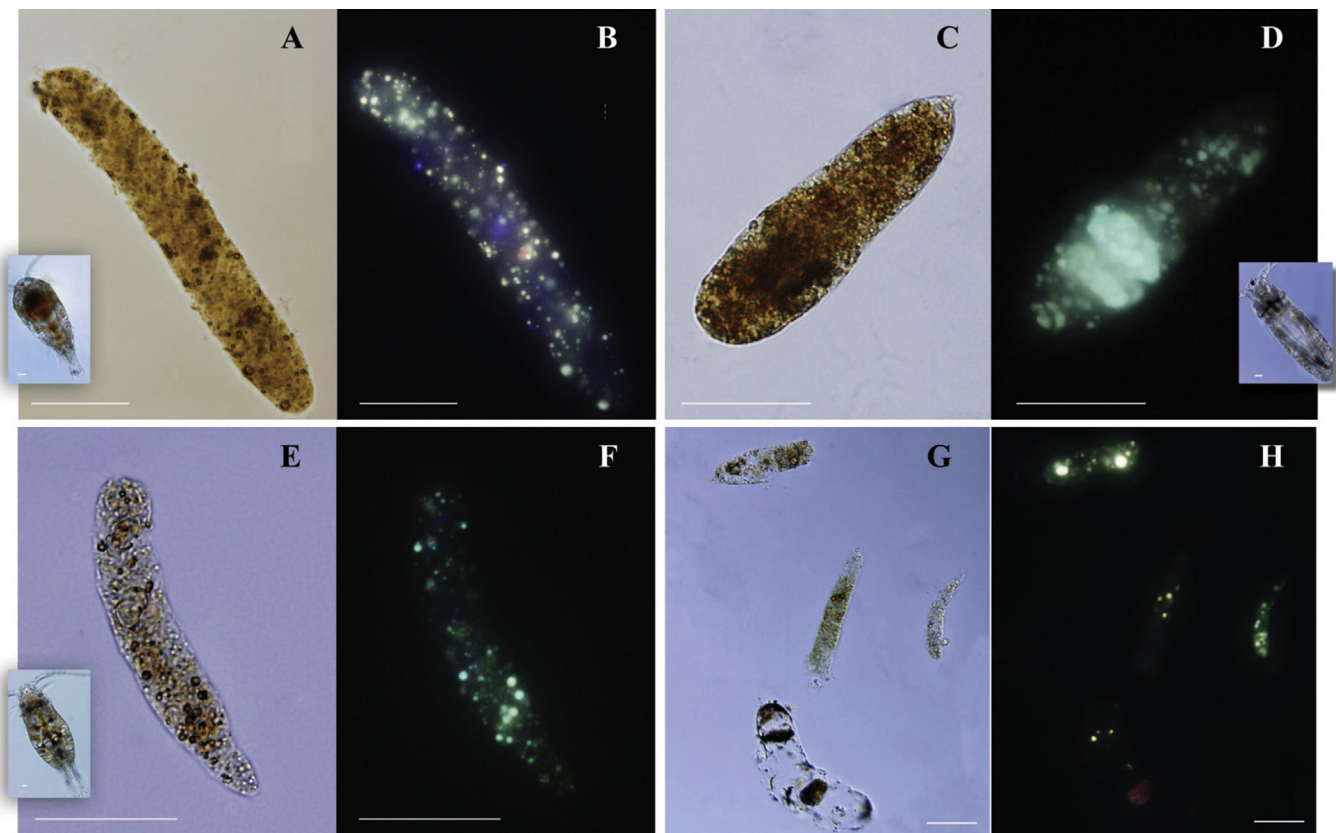
Fig. 1. Microscope images of copepod fecal pellets containing crude oil droplets. Crude oil-contaminated fecal pellets of the copepods Acartia tonsa (A–B), Temora turbinata (C–D), Parvocalanus crassirostris (E–F) and natural copepod assemblages (G–H) observed under bright (A, C, E, G) and UV illumination (B, D, F, H). Crude oil strongly autofluoresces under UV light (B, D, F, H), which was used to verify and quantify the number and volume of crude oil droplets inside the fecal pellets. Scale bar = 50 \mu\text{m} .
