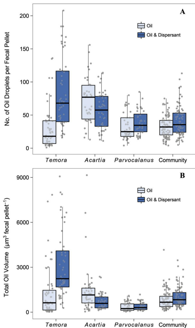
Fig. 4. Number of crude oil droplets per fecal pellet (A) and total crude oil volume per fecal pellet (B) defecated by copepods Temora turbinata , Acartia tonsa , Parvocalanus crassirostris and natural copepod assemblages (Community) that were incubated with crude oil emulsions (Oil) or chemically dispersed crude oil (Oil + Disp). Grey dots are individual data points (jittered), horizontal black bar shows the median, boxes encompass the interquartile range, and whiskers are 1.5 times the interquartile range.
