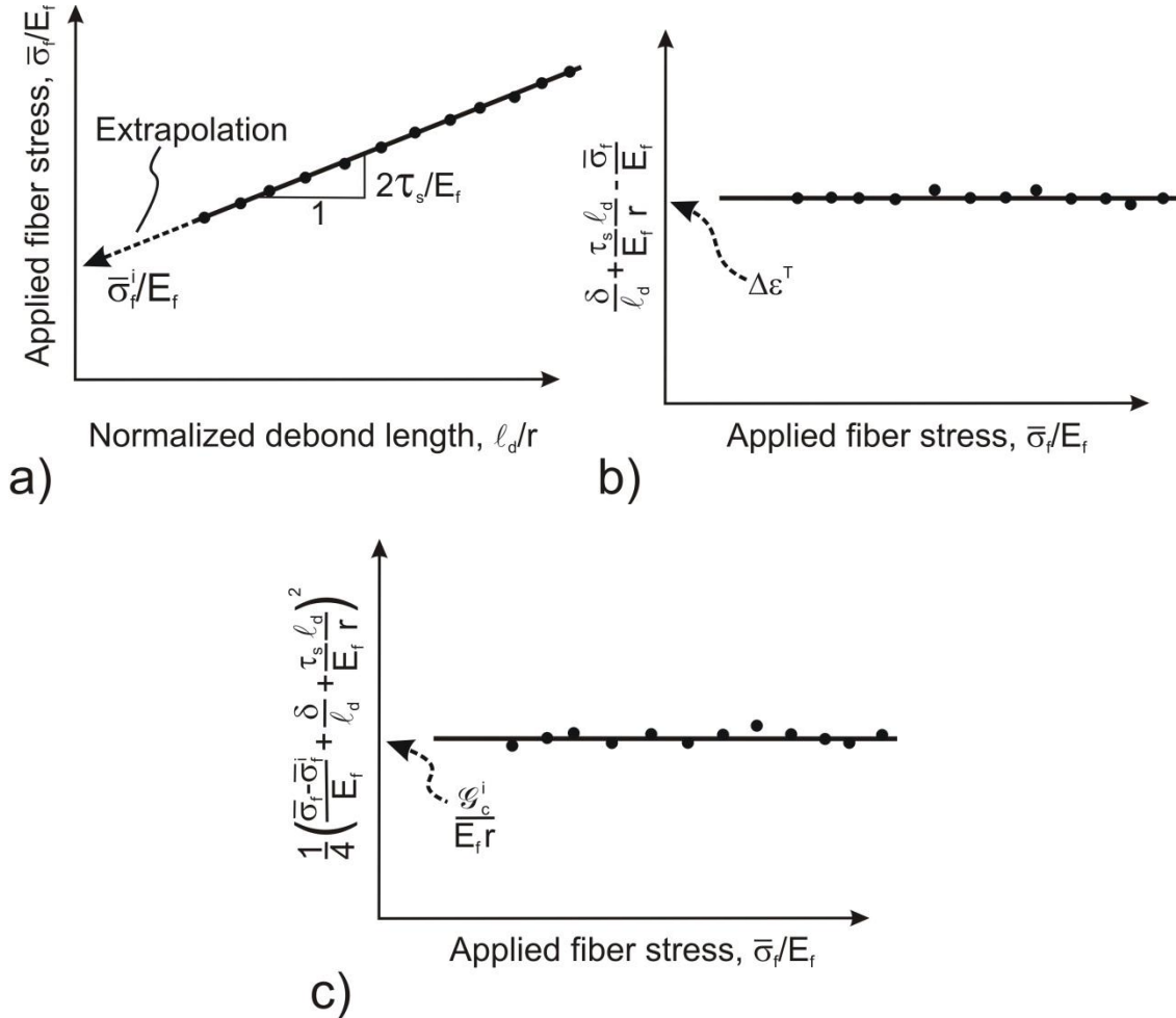
Figure 3. Sketches of plots for the determination of parameters \tau_s , \Delta\varepsilon^T and \mathcal{G}_c^i from data from pull-out experiments. (a) A plot of \bar{\sigma}_f as a function of \ell_d for the determination of \tau_s according to (21). (b) Plot of experimental values of \bar{\sigma}_f , \delta and \ell_d combined according to Eq. (25) to give \Delta\varepsilon^T . (c) Values of \bar{\sigma}_f , \delta and \ell_d combined according to (28) to give \mathcal{G}_c^i .
