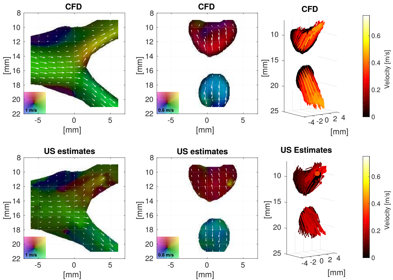
Fig. 4. Vector flow images (VFI) of the longitudinal and the cross-sectional planes, (a) and (b). A full 3-D vector representation of the cross-sectional plane is shown in (c). Reference velocities from the CFD are shown on top and estimated velocities are in the bottom. In the VFI frames the velocity magnitude and direction is represented according to the colormap in the left corner. In the full 3-D vector representation, the velocity magnitude is color encoded according to the colorbar.
