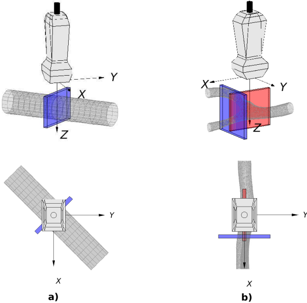
Fig. 1. Estimated planes for the simulated straight vessel (a) and the simulated CFD carotid bifurcation model (b).
