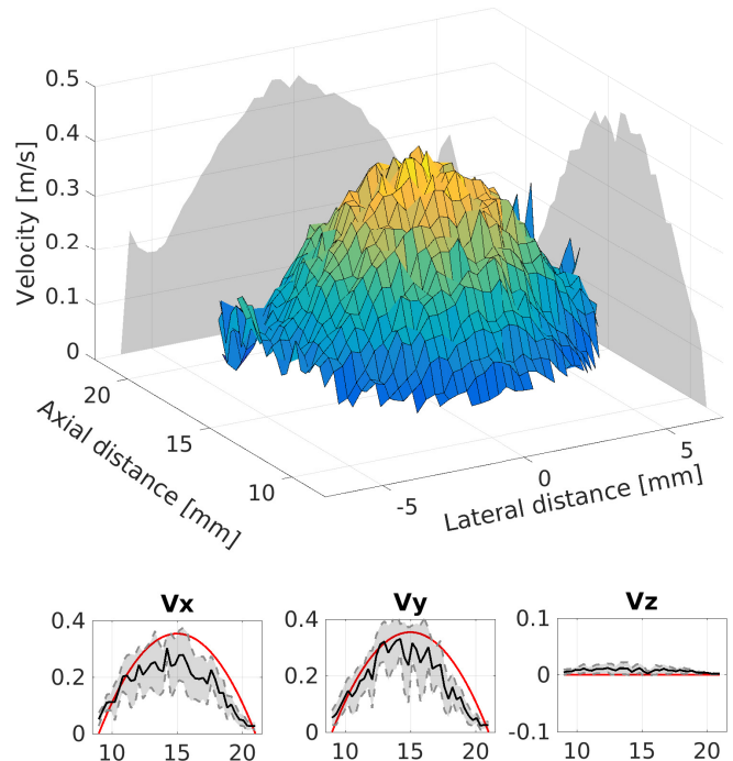
Fig. 3. Surface plot of the mean velocity magnitude across the cross-sectional plane of the straight vessel phantom (top). Mean and standard deviations (SD) of the estimated velocity components at the center line, with the true profile in red (bottom).
