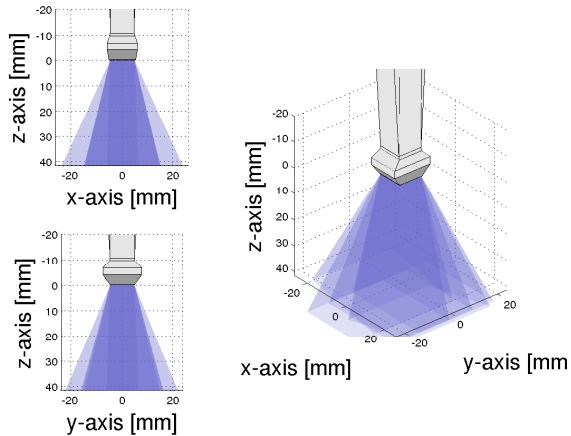
Fig. 2. Overlay of the insonified area from each emission, along the XZ and YZ plane (left), and the full volume of interest shown in a darker shade (right).
