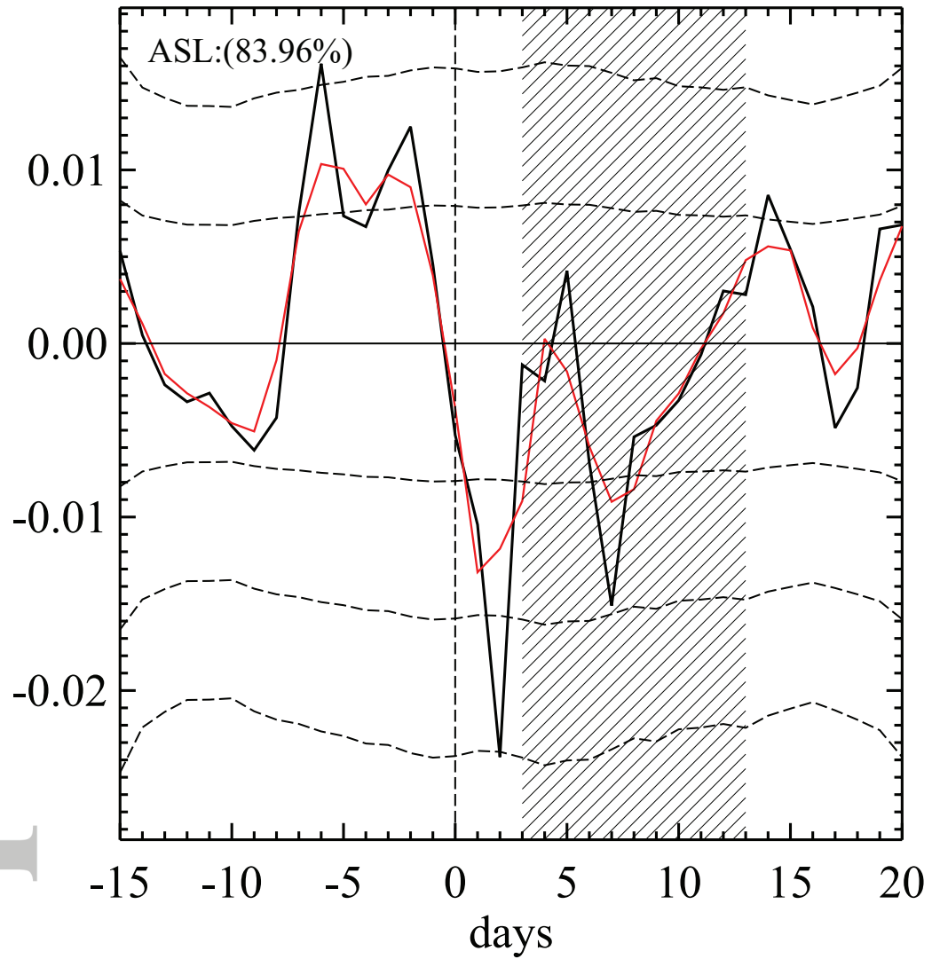
Figure 16. Cloud fraction from the ISCCP all UV data superposed over the five dates shown in Fig. 15 with maximum UV. The dashed lines denotes the n\sigma variance, with integer n .
