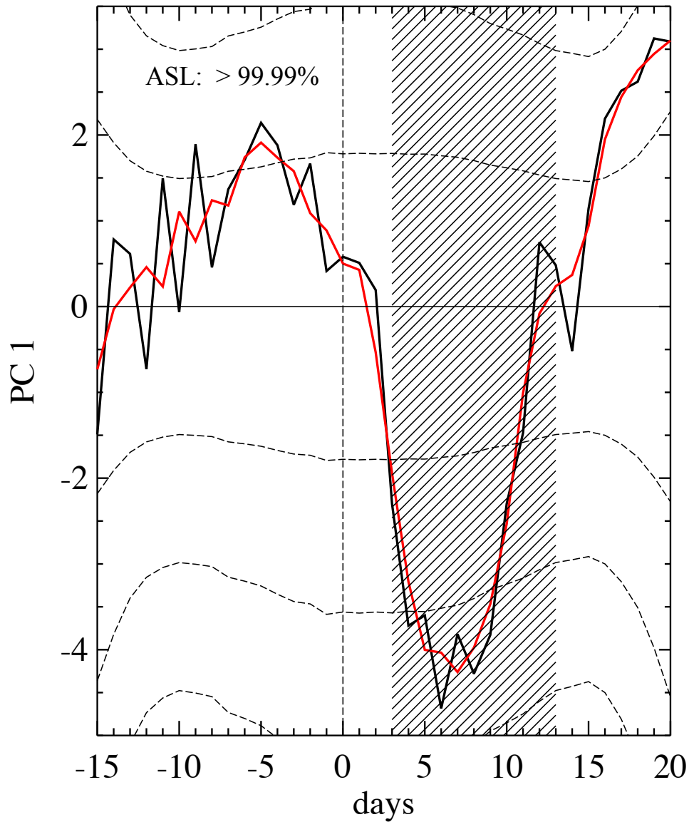
Figure 12. The first principal component (based on the six MODIS parameters, ISCCP total IR clouds over oceans and SSM/I) averaged over the 5 strongest events in the period starting with the FD on July 16., 2000. The dashed lines show 1 and 2 standard deviations, respectively. The hatched area from day 3 to day 13 is the interval over which first principal component is integrated. The achieved significance level from the integrated signal is here > 99.99\% , meaning that none of the 10^4 Monte Carlo realizations gave an absolute result of the same size or larger.
