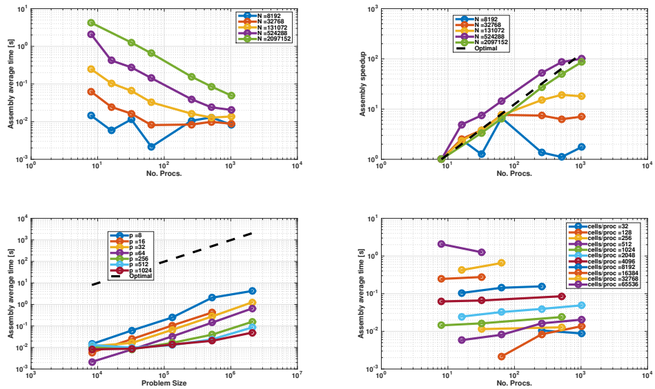
Figure 10.10: Assembly
