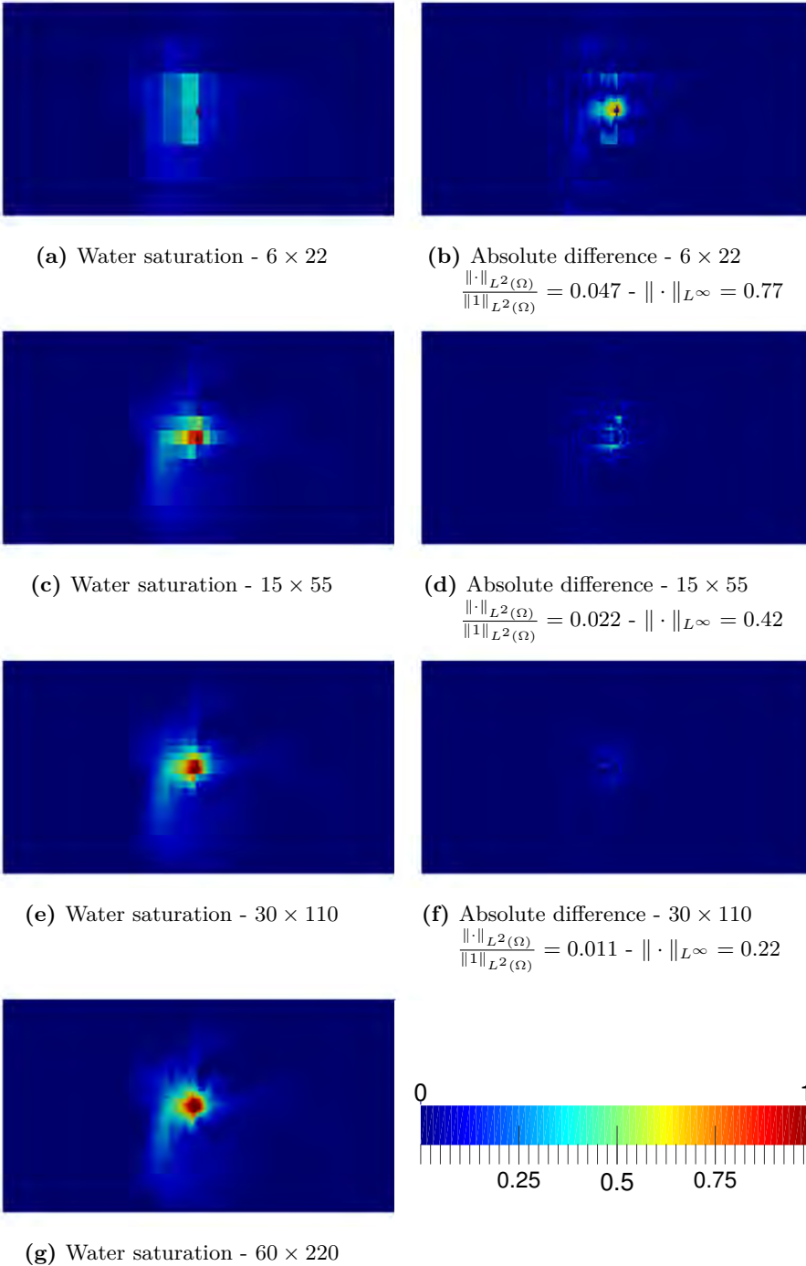
Figure 6.7: Left column: Water saturation after first water breakthrough (after 210 days) for fine grid reference solution and the 3 upscaled solutions. Right column: Absolute difference between fine grid reference solution and 3 upscaled solutions.
