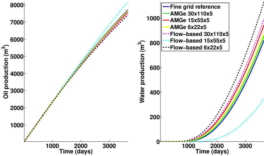
Figure 7.2: Accumulated production.
