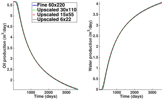
Figure 6.3: Daily production data for fine grid 60 \times 220 and upscaled models.
