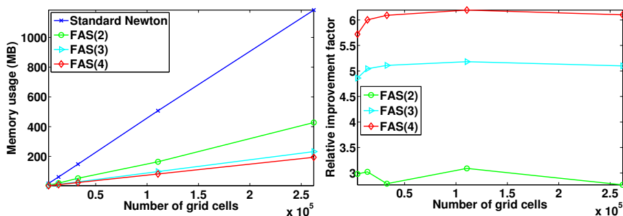
Figure 5.4: Left plot: Memory usage as a function of the number of grid cells. Right plot: Relative improvement for FAS( \ell ) over SN.
