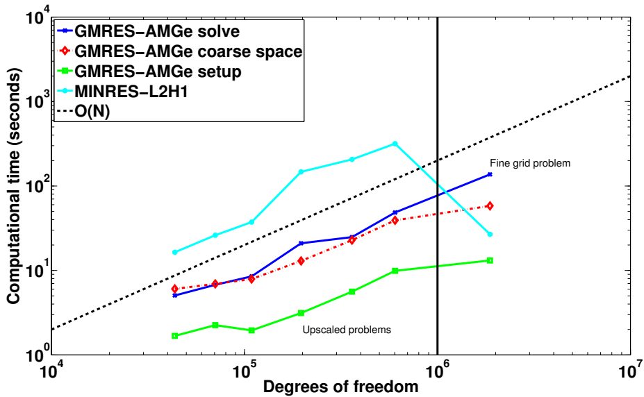
Figure 7.5: Computational time vs degrees of freedom for AMGe and L_2 - H^1 preconditioning of the upscaled systems.
