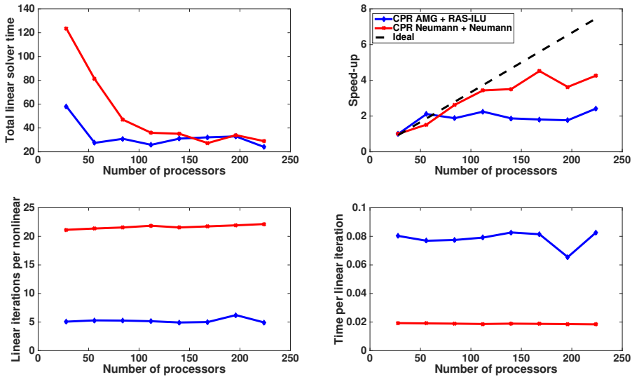
Figure 10.15: Strong scaling
