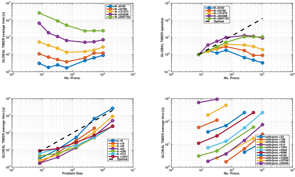
Figure 10.3: Global timer
