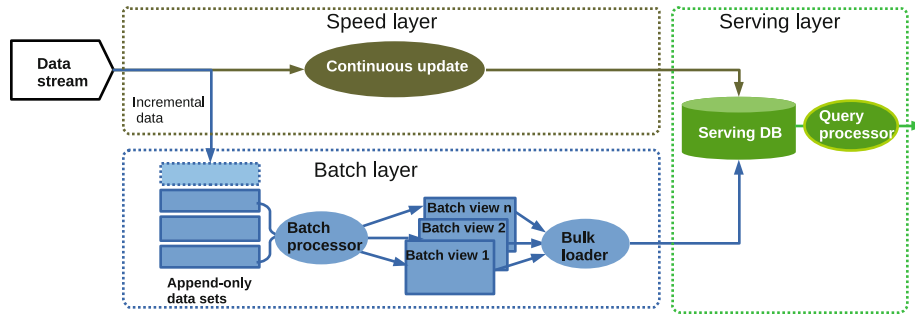
Fig. 2. Lambda architecture
