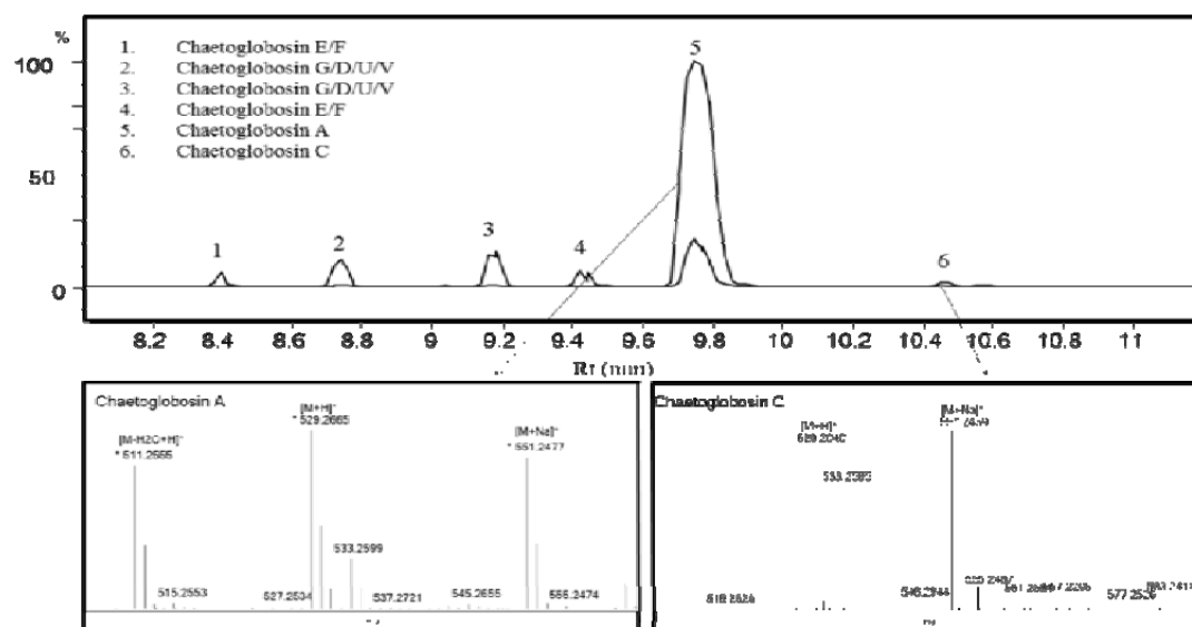
Fig. 3 Combined extracted ion chromatograms of m/z 529.2697 corresponding to pseudomolecular ion of chaetoglobosin A, C, G, D, U and/or V resulting in four peaks: 2, 3, 5 and 6; and of m/z 531.2853 corresponding to pseudomolecular ion of chaetoglobosin E and F (peaks 1 and 4). MS spectra of identified chaetoglobosin A (peak 5) and C (peak 6) were presented below
