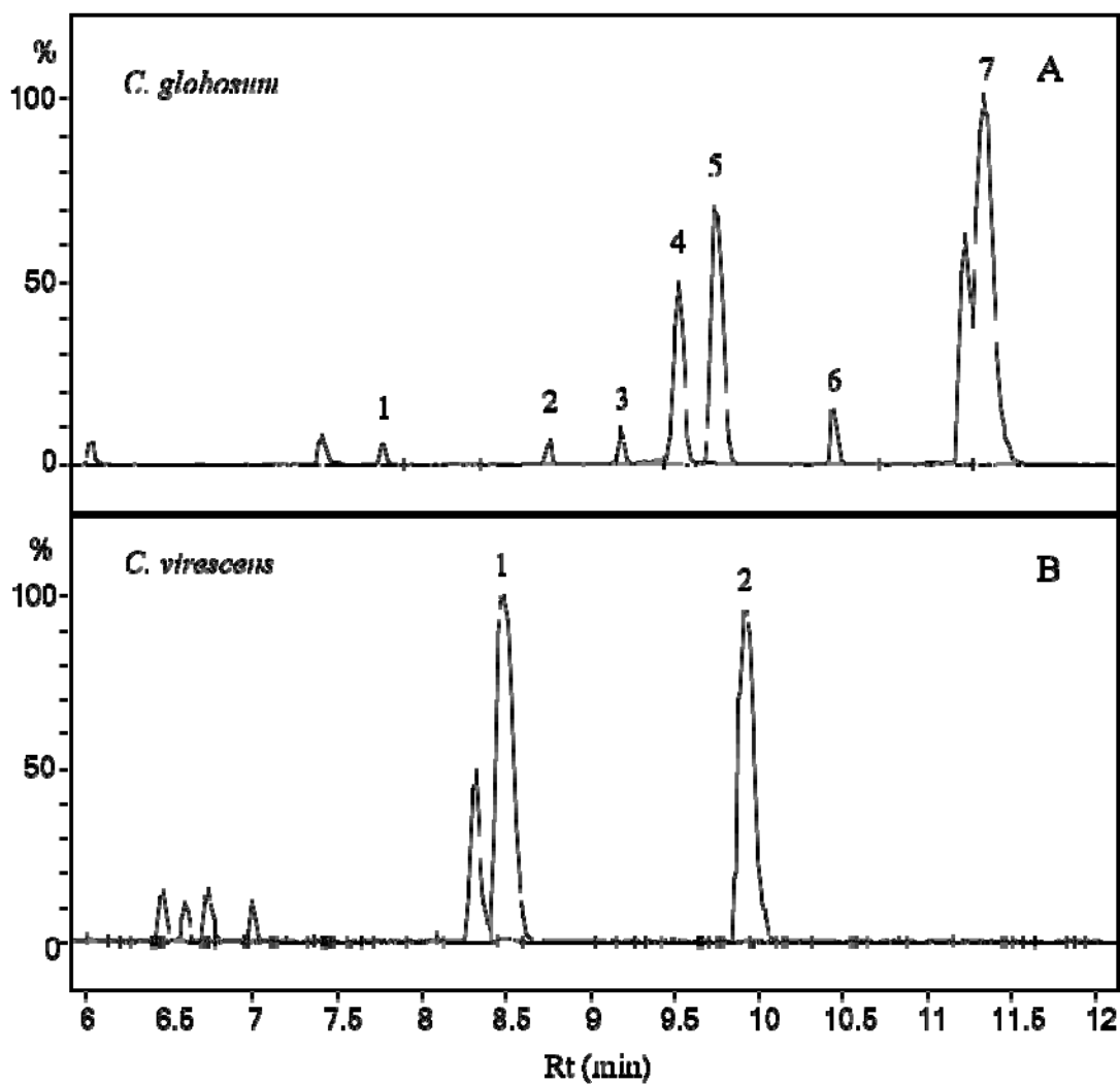
Fig. 5 Comparison of combined extracted ion chromatograms (6-12 min) of indoor ( C. globosum , IBT 41801) and reference strain ( C. virescens , IBT 26237) MEA extracts: A: C. globosum 1 – cochliodone 1, 2 – chaetoglobosin G/D/U/V, 3 – chaetoglobosin G/D/U/V, 4 – cochliodone 2, 5 – chaetoglobosin A, 6 – chaetoglobosin C, 7 – cochliodone 3; B: C. virescens 1 – 3-O-methylsterigmatocystin, 2 – sterigmatocystin
