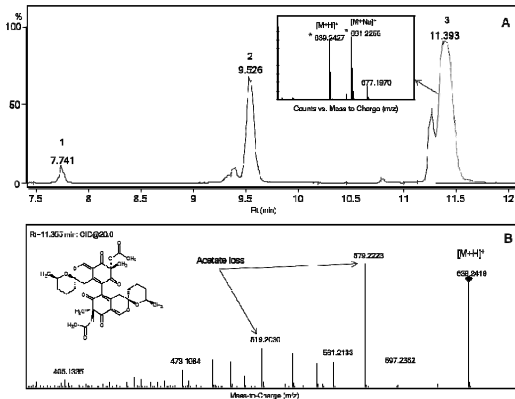
Fig. 4 Chromatogram (A) of three peaks identified as 1 – cochliodone 1 (Rt 7.74 min), 2 – cochliodone 2 (Rt 9.52 min) and 3 – cochliodone 3 (Rt 11.39 min) together with MS/MS spectrum of cochliodone 3 at 20 eV (B)
