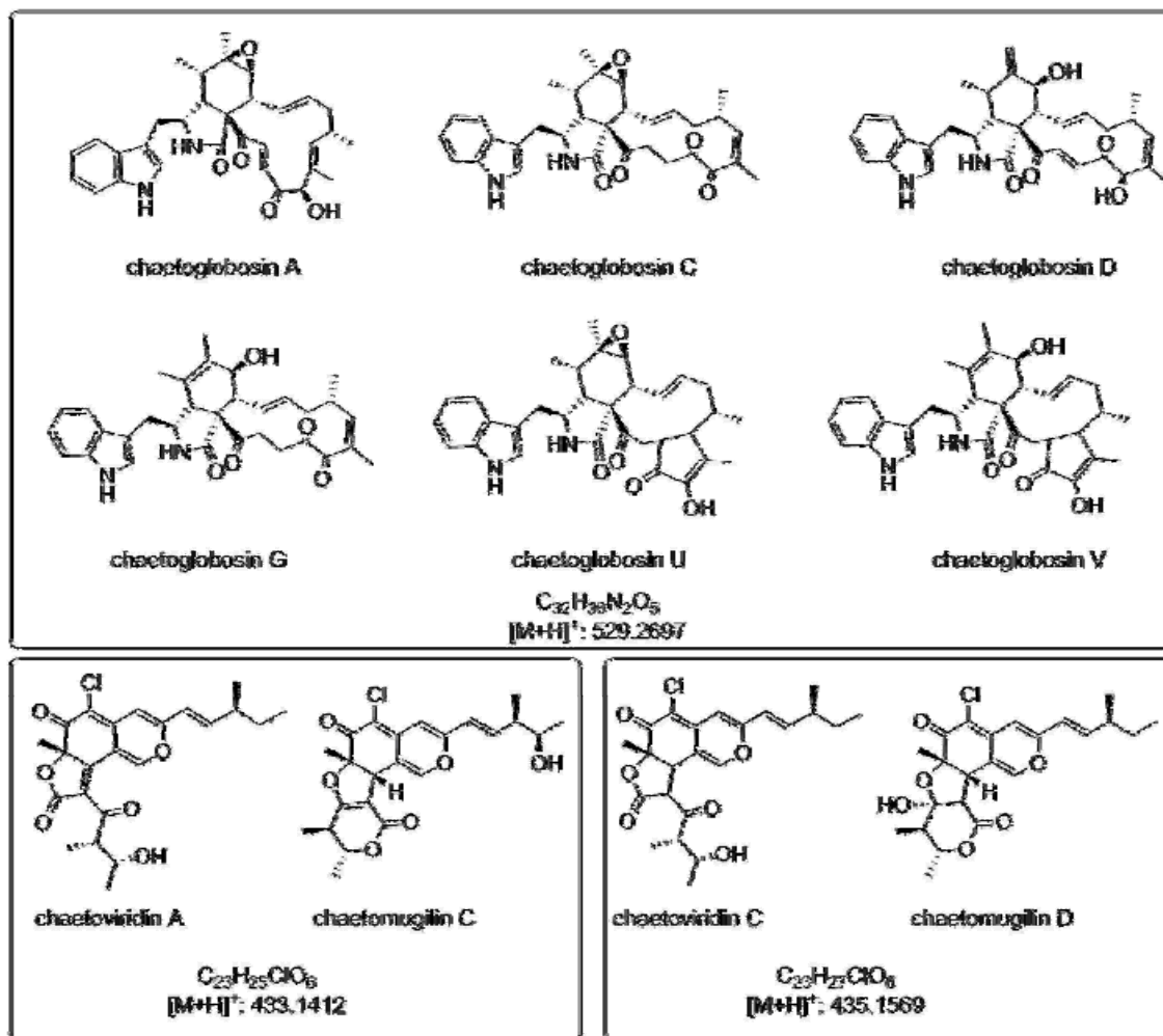
Fig. 1 Chemical structures of chaetoglobosins, chaetoviridins and chaetomugilins with the same elemental composition found in C. globosum
