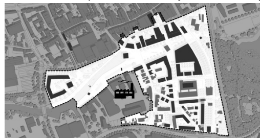
Fig. 4: Investigated area (light coloured) with old building stock (grey), new developments (black) and waste heat sources (icon).
