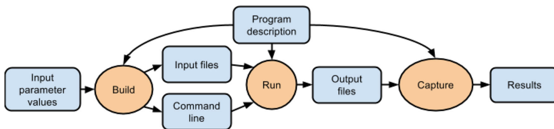
Fig. 1 Wrapping mechanism that transforms a user's request into the execution of a command-line tool in Mobyale
