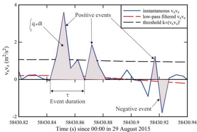
Figure 2. Momentum flux data collected on 29 August 2015 and turbulent flux event definitions
