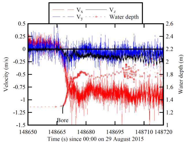
Figure 4. Time-variation of free-surface elevation and instantaneous velocity components during the tidal bore of the Garonne River (France) on 30 August 2015.
