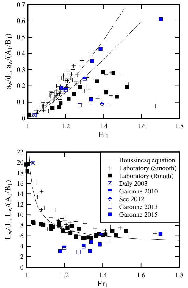
Figure 3. Free-surface characteristics of the undular tidal bore of the Garonne River (France). Top: secondary wave amplitude; Bottom: secondary wave length. Comparison between laboratory data on smooth and rough beds, and field observations. Same legend for both graphs
