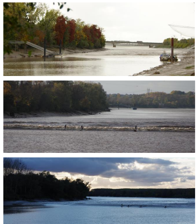
Figure 1. Tidal bore of the Garonne River (France) on 28 October 2015. Top: Arcins at 16:24 - note the pontoon on right where velocimeter was installed; Middle: Cambes, 29 min later and 9.6 km upstream of Arcins; Bottom: Langoiran, 21 min later and 6.6 km upstream of Cambes.
