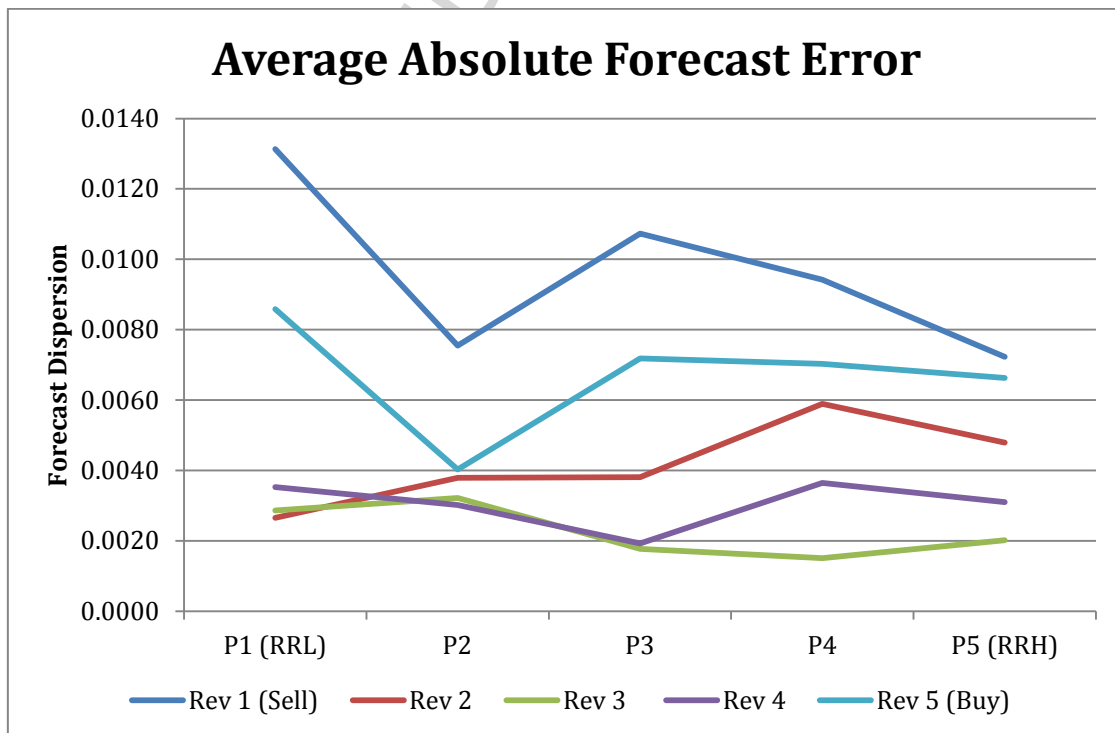
Figure 2 Average Analysts' Performance (Absolute Forecast Error)
