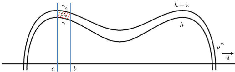
Fig. 4 Section \Omega in which H^{-1}(h) is transverse to p
