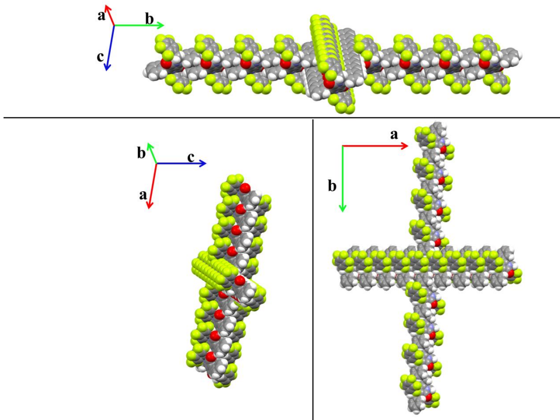
Figure 2. Illustration of the cruciform supramolecular arrangement observed in HHFBDPP .
