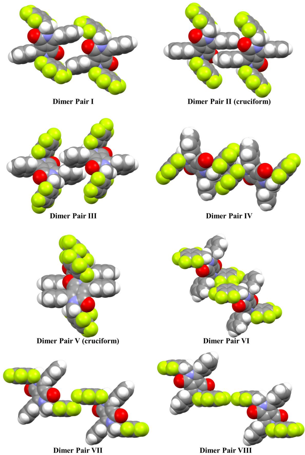
Figure 3. Space filled representation of all the nearest neighbour dimer pairs of HHFBDDPP .
