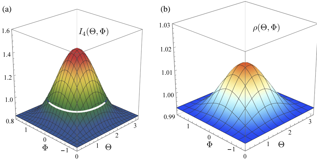
Figure 4: Surface contour plots of (a) I_4(\Theta, \Phi) and (b) \rho(\Theta, \Phi) for a uniaxial tension test within the half sphere \mathbb{S} = \{(\Theta, \Phi) \mid \Theta \in [0, \pi], \Phi \in [-\pi/2, \pi/2]\} , defined with respect to a local coordinate system constructed from the eigenvectors of \mathbf{C} ( b = 0.01 , \lambda = 1.2 ). The small gap in (a) represents the plane where I_4 = 1 . Thus, only the fibers located within the domain enclosed by the gap are extended. In either plot, the center point ( \Theta = \pi/2 , \Phi = 0 ) represents the mean fiber orientation along the \mathbf{V}_1 axis in the local coordinate system, which is coincident with the \mathbf{E}_3 axis in the global Cartesian coordinate system; the line at \Theta = 0 represents the \mathbf{V}_3 axis on the unit sphere; the point located at \Theta = \pi/2 and \Phi = \pi/2 represents the \mathbf{V}_2 axis on the unit sphere.
