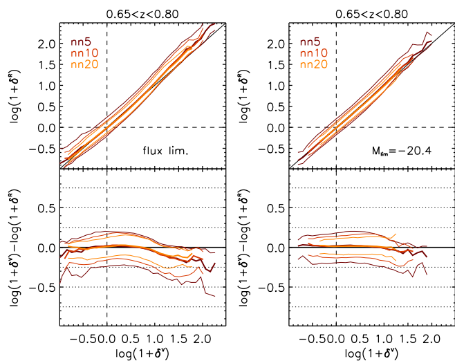
Fig. A.2. Comparison of \delta^R and \delta^V on a galaxy-by-galaxy basis. Results are shown for the cylindrical filter with radius corresponding to the fifth, tenth, and twentieth n.n. for the redshift bin 0.65 < z < 0.8 . The density is computed using flux-limited tracers (left) and volume-limited tracers with M_{lim} = -20.4 (right). x -axis: density contrast in the Vmocks; y -axis, top panel: density contrast in the Rmocks; y -axis, bottom panel: difference of the logarithms. The thick lines are the median value of the quantity displayed on the y -axis in each x -axis bin. Thin lines represent the sixteenth and eightyfourth percentiles of its distribution. The solid black line in the top panels is the one-to-one line, and the horizontal lines in the bottom panels are for reference.
