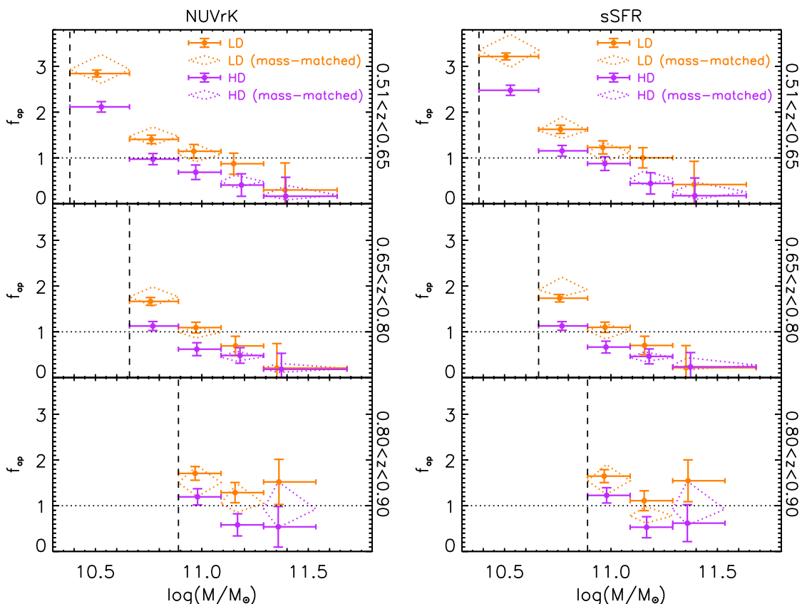
Fig. 5. Ratio of the number of active over passive galaxies ( f_{ap} ) in LD (orange filled circles) and HD (violet filled circles) regions as a function of stellar mass in three different redshift bins. Active and passive galaxies are defined by means of the NUVrK diagram ( left ) or according to their sSFR ( right ). Horizontal error bars indicate the span of the mass bin, and the vertical error bars are derived from the propagation of the Poissonian noise in the counts of active and passive galaxies (if we use the error formula for small samples suggested in Gehrels 1986, the error bars do not change significantly). The x -axis value is the median stellar mass of the sample used to compute f_{ap} . Dotted diamonds are for the mass-matched samples in the environment (LD or HD) with more galaxies in each mass and redshift bin. Diamonds are centred on the median f_{ap} value of the 100 mass-matched extractions, and the bottom and top vertices represent the 25% and 75% of the f_{ap} distribution, respectively. The x -axis values is the median of the median stellar mass in each extraction. See text for more details. The vertical dashed line in each redshift bin is the corresponding mass limit M_{lim} . The dotted horizontal line at f_{ap} = 1 is for reference.
