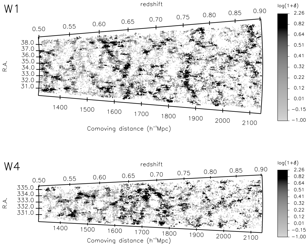
Fig. 1. R.A. – z distribution of secure-redshift galaxies in W1 (top) and W4 (below), in comoving coordinates. For the sake of clarity, only the central degree in Dec is plotted. The colour used for each galaxy refers to the value of the local density computed around the galaxy (from light grey for the lowest density to black for the highest density, as in the colour bar). The density is computed in cylindrical filters with radius corresponding to the fifth n.n., using the volume-limited sample of tracers that is complete up to z = 0.9 .
