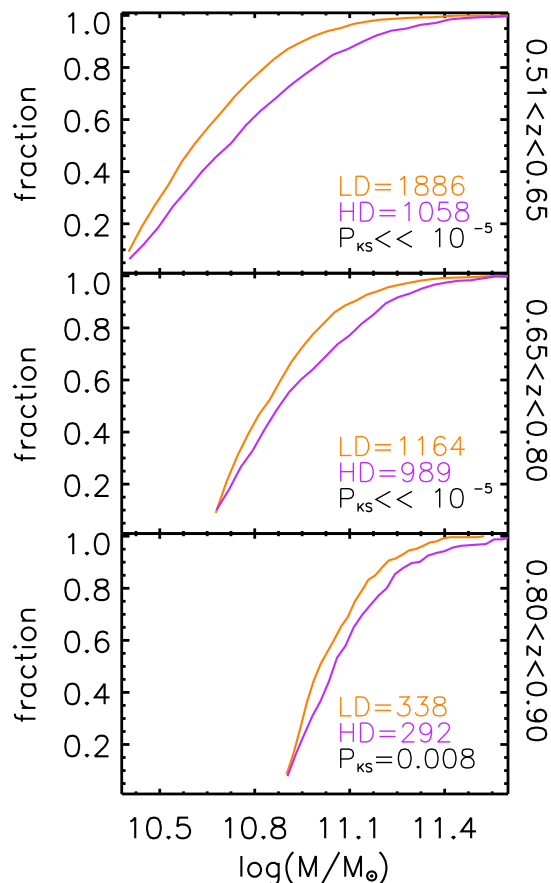
Fig. 4. Stellar mass cumulative distributions in three redshift bins ( 0.51 < z \leq 0.65 , 0.65 < z \leq 0.8 , and 0.8 < z \leq 0.9 from top to bottom), for galaxies above the mass limits \log(M_{lim}/M_{\odot}) = 10.38 , 10.66, and 10.89, respectively, in the three redshift bins. Orange lines show the galaxies in LD regions, and violet lines show galaxies in HD regions. The number of galaxies used in each distribution is reported in the corresponding panel. We use all the galaxies above the mass limit, regardless of their NUVrK classification. In each panel we also report the P_{KS} values, i.e. the significance level in a Kolmogorov-Smirnov test for the null hypothesis that the LD and HD distributions are drawn from the same parent distribution.
