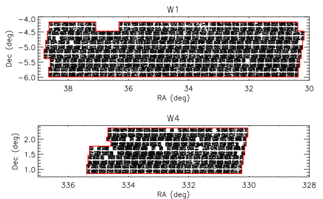
Fig. A.1. R.A.-Dec distribution of secure redshift galaxies in W1 (top) and W4 (below). The red thick line in each panel is the ‘field boundary’ that we consider in this work. The cross-like pattern of void regions is due to the characteristic footprint of the VIMOS instrument. Rectangular empty regions are missing quadrants that have been discarded due to too poor observational conditions or technical problems.
