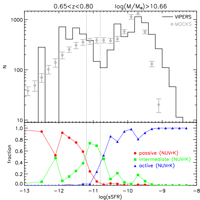
Fig. 3. Top. Black histogram: distribution of the sSFR ( = SFR/M ) for the VIPERS galaxies in the redshift range 0.65 < z < 0.8 and for \log(M_{lim}/M_{\odot}) > 10.66 , which is the completeness mass limit in that redshift range. Diamonds: sSFR distribution in the RMOCKS for galaxies in the same redshift range and above the same mass threshold; the points with the vertical error bars correspond to the average and rms of the 50 mocks catalogues. The sSFR distribution of the RMOCKS is normalised to have the same total number of galaxies as in the VIPERS sSFR distribution. Both the real and simulated distributions have a tail of galaxies with sSFR values below the lowest sSFR limit in this plot, which we do not plot for the sake of clarity. Bottom. Only for the VIPERS sample (same galaxies as in the top panel), fraction of passive (red circles) and active (blue triangles) galaxies as defined by Eqs. 3 and 4, as a function of their sSFR . We also overplot the fraction of ‘intermediate’ galaxies, i.e. those that do not satisfy the passive or the active definition. The vertical lines at \log(sSFR) = -11.2 and \log(sSFR) = -10.8 are the thresholds adopted to define passive and active galaxies, respectively, using the sSFR as discussed in Sect. 4.1. These results are very similar in the two other redshift bins (not shown).
