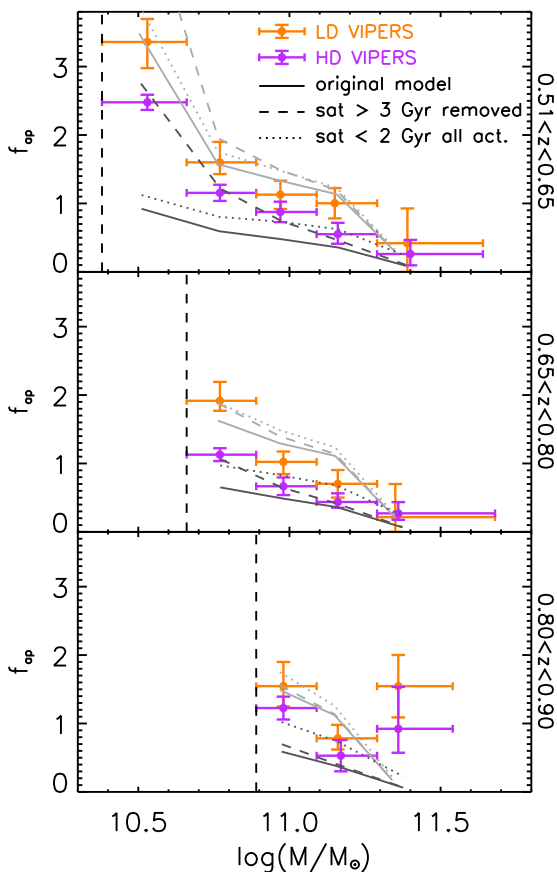
Fig. 9. Fraction f_{\text{ap}} in the VIPERS data (orange and violet crosses) and in the model (grey lines). Crosses are the same as in Fig. 7. Solid grey lines refer to Rmocks and correspond to the grey polygons of Fig. 6. Dashed lines refer to Rmocks, but are computed after removing satellite galaxies that became satellites more than 3 Gyr before. The dotted lines refer to Rmocks, but are computed considering all the ‘young’ satellite galaxies (i.e., that became satellites less than 2 Gyr before) to be active. See the text for more details.
