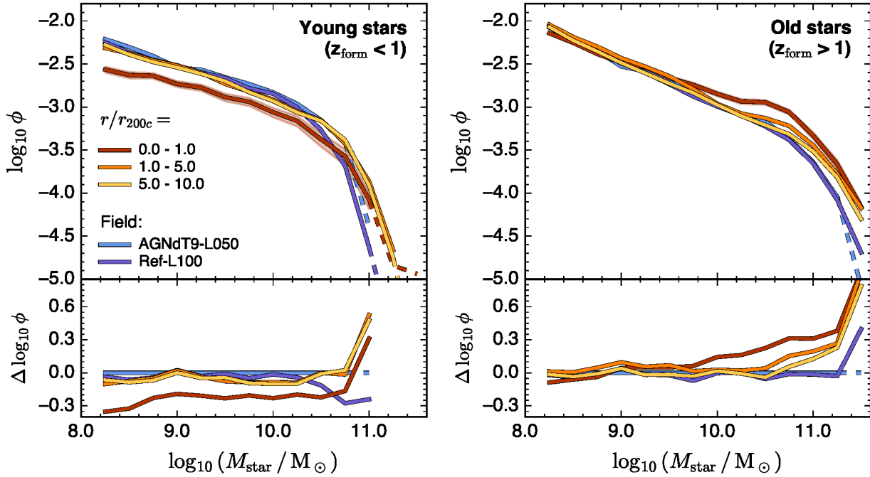
Figure 8. Top panels: the normalized z = 0 galaxy stellar mass functions \phi \equiv dn/d\log_{10} M_{\text{star}}/(M_{\text{tot}}/10^{10}M_{\odot}) split by stellar formation redshift into ‘young’ stars ( z_{\text{form}} < 1.0 , left-hand panel) and ‘old’ stars ( z_{\text{form}} > 1.0 , right-hand panel). As in Fig. 7, the Hydrangea volumes are split into three radial zones (red, orange, and yellow lines) and compared to the EAGLE periodic-box simulations (blue/purple); dashed lines indicate bins with fewer than ten galaxies. The shaded band, shown only for r < r_{200c} (red) for clarity, indicates the Poisson uncertainty on the GSMF. For clarity, the bottom panels show the logarithmic ratio between each GSMF and that from the AGNdT9-L050 periodic box. Evidently, the deficiency at low mass and excess of stellar mass at high mass are due to two different processes, since the former only affects young, and the latter mostly old stars.
