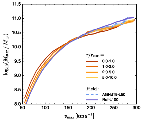
Figure 11. Stellar mass of Hydrangea galaxies as a function of maximum circular velocity, v_{\text{max}} , compared to the field (blue/purple). In contrast to the comparison at fixed total mass presented in Fig. 10, there is no strong environmental offset for massive galaxies, with a small deficit of stellar mass in massive cluster galaxies compared to field galaxies of the same v_{\text{max}} .
