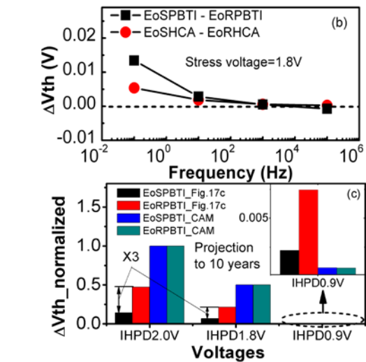
Fig. 18 EoSPBTI-EoRPBTI & EoSHCA-EoRHCA at (a) 2.0V and 1.8V are constant, confirming they are from PCET. (b) Its frequency dependency. PCET causes the 'n' variation in Fig.17c. (c) \Delta V_{th} prediction to 10 years by conventional extrapolation (data is from Fig. 17c) and CAM model.
