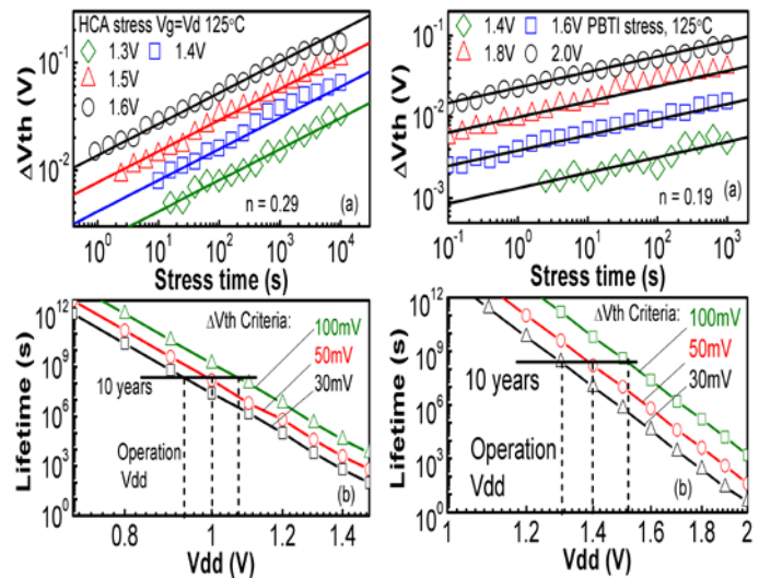
Fig. 1 Conventional power-law method for HCA lifetime prediction. (a) V th degradation at accelerated V g =V d . (b) V th degradation at accelerated V g . (b) V dd extrapolation for 10 years lifetime based on different \Delta V_{th} criteria.
