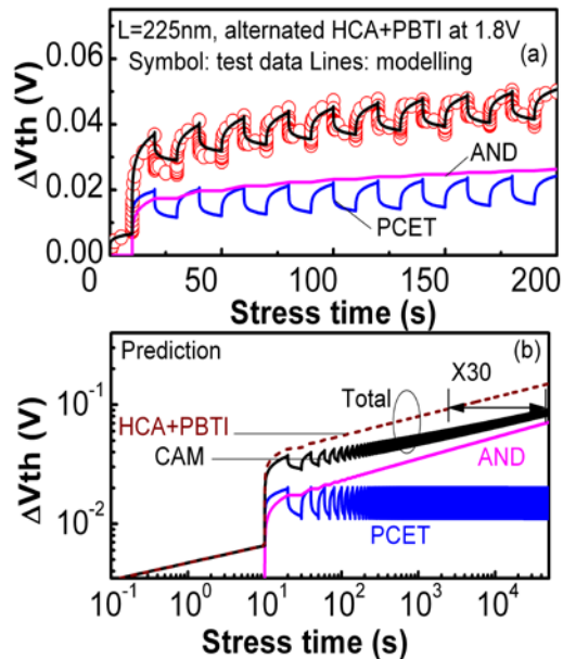
Fig. 5 Test results and modelling for short channel device at 1.8V (a) for IHPD. Lifetime prediction with V_{th}=100mV (b) and operation Vdd for 10 years (c) based on CAM framework
