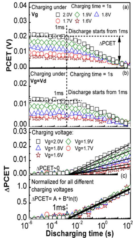
Fig. 12 Modelling for PCET discharging ( V_d mode). PCET is charged for 1s under (a) V_g -only, and (b) under V_g=V_d conditions. (c) The discharged \Delta PCET follows logarithmic law against discharging time and can be normalized to a unique kinetics.
