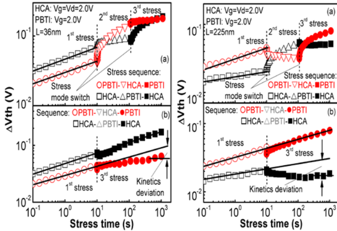
Fig. 3 (a) Alternating HCA-PBTI in short-channel device. Sequence: HCA-PBTI-HCA and PBTI-HCA-PBTI. (b) The 2 nd stress is removed, and both \Delta V_{th} and stress time of the 3 rd stress are reset to that at end of the 1 st stress.
