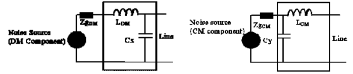
Fig. 4. a) typical DM filter b) typical CM filter
