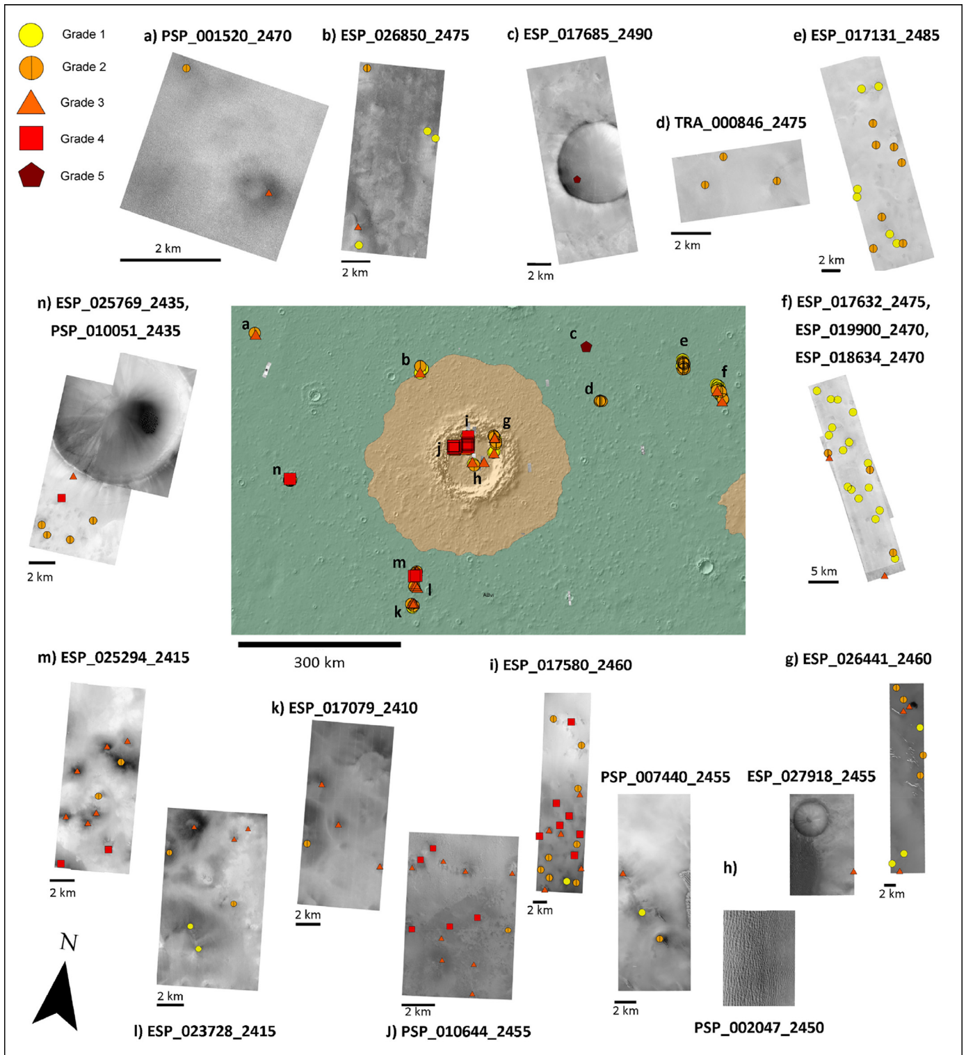
Fig. 6. Results of the boulder patch classification. Each inset shows the distribution of graded features within one or more HiRISE images (NASA/JPL/University of Arizona). The central image shows site locations overlain on the geological map of the Martian Northern Plains (Tanaka et al., 2005), which illustrates the extent of the Lomonosov crater ejecta blanket. 17 Images exhibit features.
