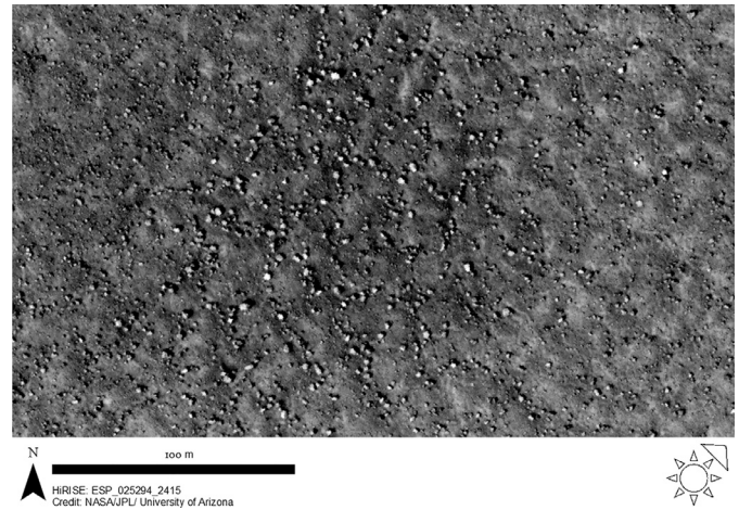
Fig. 8. Net of less dense discontinuous polygons in HiRISE image ESP_025294_2415, covering flat ground to the south of Lomonosov crater.
