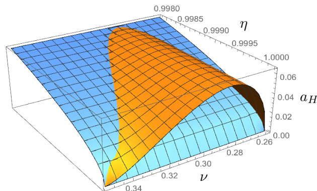
Figure 5. a_H versus (\nu, \eta) for \frac{1}{2}\sqrt{2 - \sqrt{3}} < \nu < 1/(2\sqrt{2}) and 0.998 < \eta < 1 . The blue surface is the BMPV solution and the orange one is the black hole and bubble solution.
