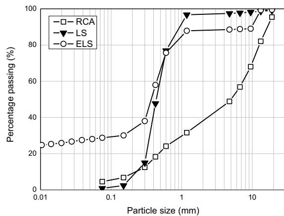
Figure 1: Particle Size Distributions for RCA, LS and ELS.
