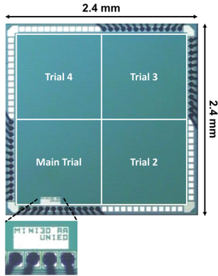
Fig. 1. Micrograph of top tier showing the 4 independent trials and the line name.
