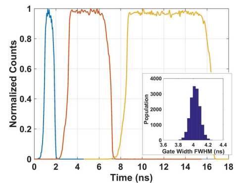
Fig. 7. 1ns, 4ns and 8ns FWHM time gate profiles of bin1 of a selected pixel. Inset is histogram of the 4ns gate width across the array with 64ps standard deviation.
