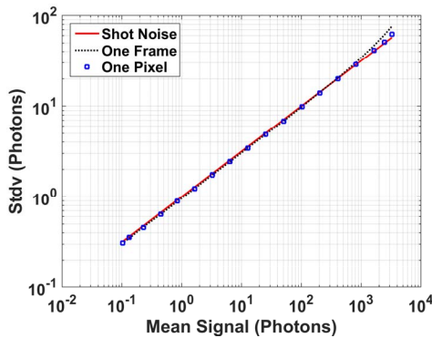
Fig. 14. Photon transfer curve of a selected pixel and a selected frame showing shot-noise limited response. Right are histograms of the selected pixel signal values at 20ns exposure (top) and 8μs exposure (bottom) with Poisson fit overlaid as crosses.
