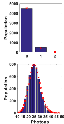
Fig. 14. Photon transfer curve of a selected pixel and a selected frame showing shot-noise limited response. Right are histograms of the selected pixel signal values at 20ns exposure (top) and 8μs exposure (bottom) with Poisson fit overlaid as crosses.
