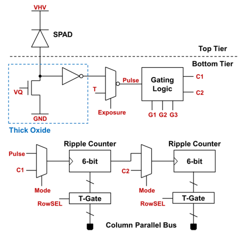
Fig. 5. Pixel circuit diagram.
