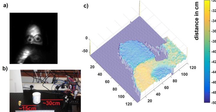
Fig. 6. Indirect time of flight experiment with 4ns laser pulse width, a) is intensity image of sensor's field of view, b) is bench setup and c) is resolved depth map with median filter applied showing a toy behind a mug's handle.
