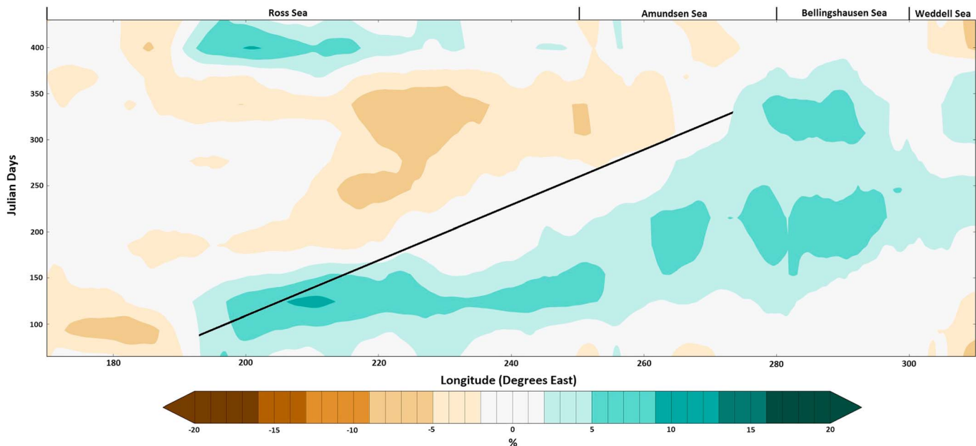
Figure 2. A Hovmöller diagram showing the changes in sea ice concentration anomalies due to El Niño from Bootstrap2 data as a function of time and longitude. The anomaly is averaged over the latitudes 60°S to 75°S. The ice drift speed was calculated based on the seasonal progression of the positive anomaly which was calculated between 195° and 275° over the course of 230 days, denoted by the solid black line. The final value was calculated based on using a value of 38,186 m per degree of longitude.
