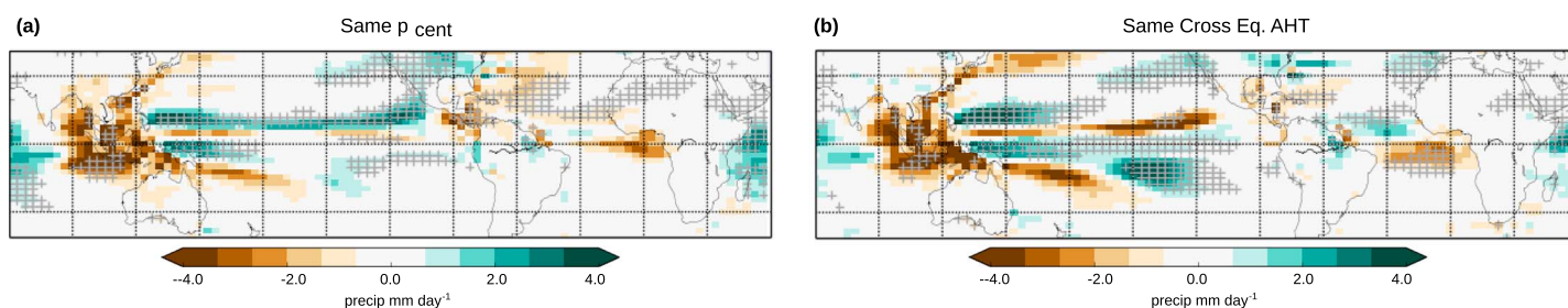
Figure 2. Difference maps of annual average precipitation between two simulations with the same (a) p_{cent} and (b) AHT. The regions marked with crosses indicate that the precipitation differs by more than 50% between the two simulations.
