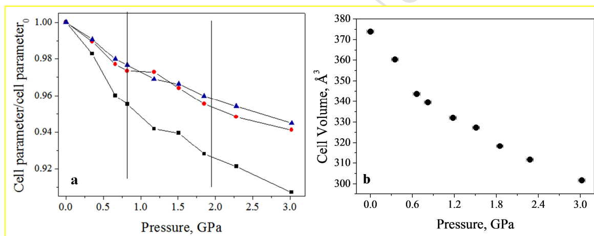
Figure 5(a) Compression plot of cell parameters for CH 3 NH 2 BH 3 as a function of pressure: black square – a/a_0 , red circle: b/b_0 and blue triangle – c/c_0 . Note data points are connected by straight lines as a visual guide. (b) Variation of the unit cell volume of CH 3 NH 2 BH 3 as a function of pressure
