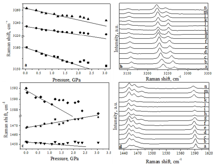
Figure 2 Changes in the Raman spectra for methylamine borane with respect to pressure (a) 3130-3350 \text{cm}^{-1} region ▲ \text{NH}_2 asymmetric stretch, ● \text{NH}_2 symmetric stretch, and ■ \text{BH}_3 symmetric stretch + \text{NH}_2\text{-BH}_3\text{-CH}_3 wag, (c) 1430-1620 \text{cm}^{-1} region ◆ \text{NH}_2 scissor, ★ \text{CH}_3 scissoring, and ▼ \text{CH}_3 twist, (b) and (d) pressure range (in GPa): a:0; b:0.04; c:0.4; d:0.6; e:0.8; f:1.1; g:1.2; h:1.4; i:1.6; j:1.8; k:2.1; l:2.2; m:2.4; n:3.0
