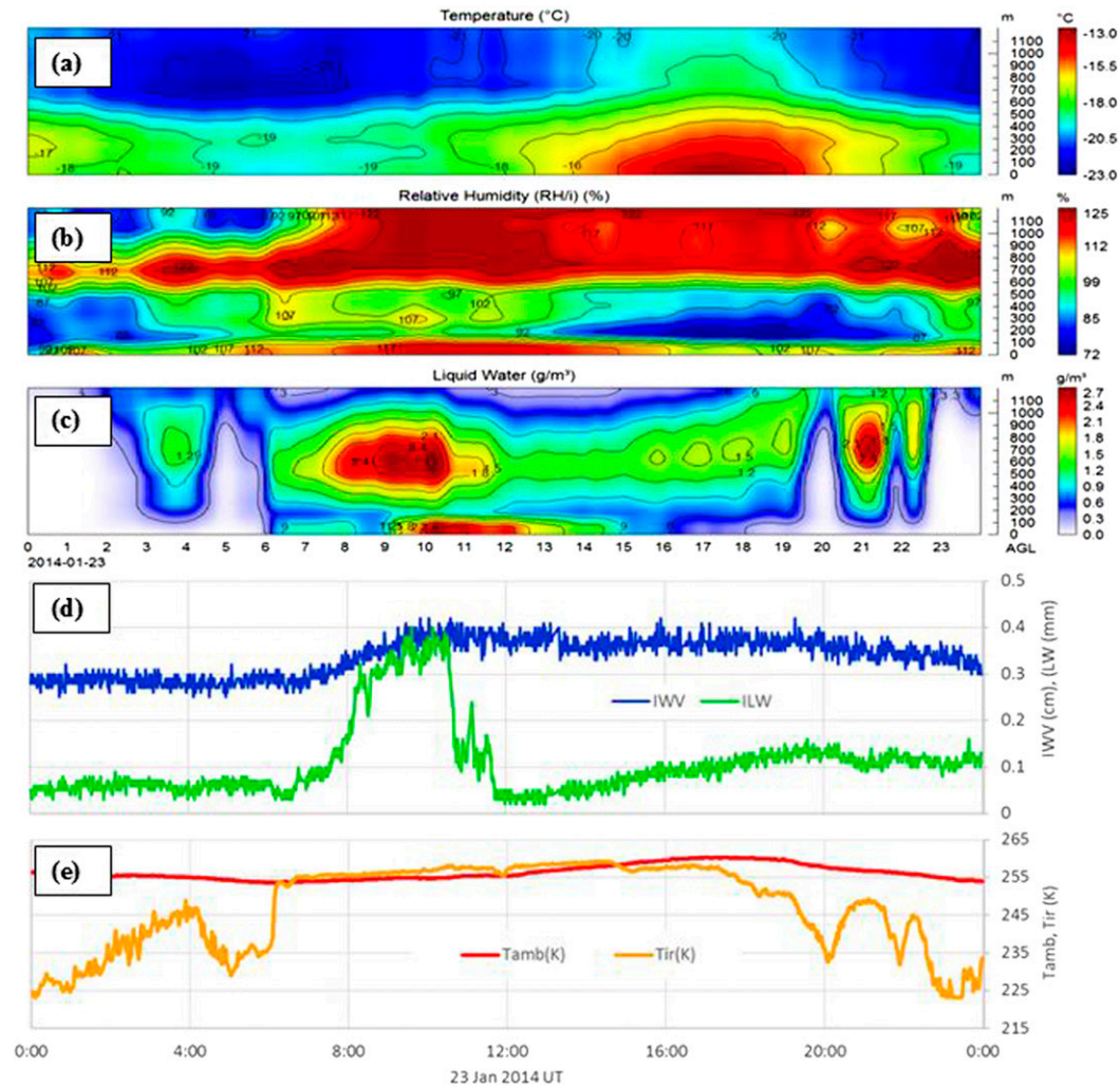
FIG. 6-6. Radiometrics PMWR (a) temperature, (b) RH over ice, and (c) LWC ( \times 10 ) profile retrievals to 1.2-km height, (d) IWV and ILW retrievals, and (e) surface temperature ( T_{amb} ) and cloud-base IR temperature ( T_{ir} ) for 23 Jan 2014.
