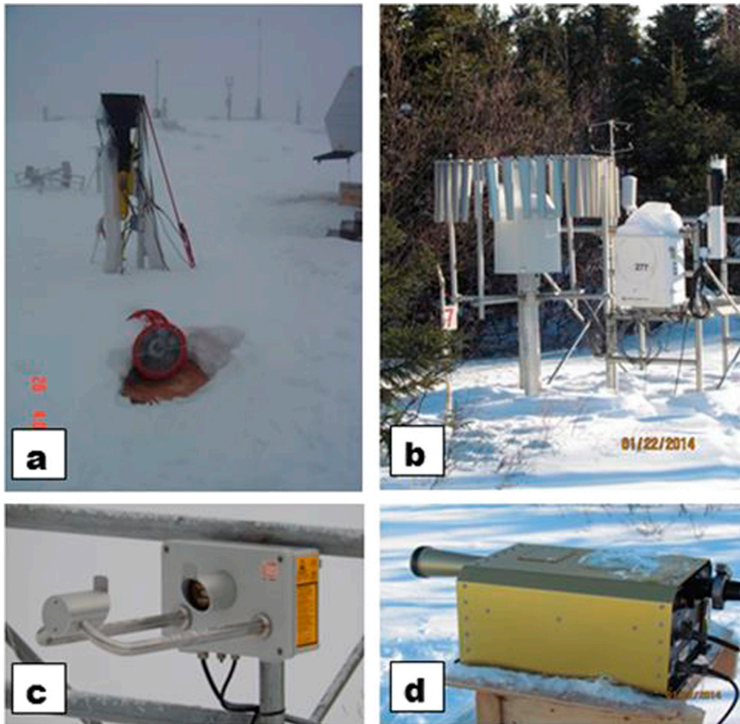
FIG. 6-4. (a) GCIPI instrument for snow spectral measurements at sizes less than about 1 mm. (b) Pluvio instrument with a single-alter shield at 3-m height with a Metek Inc. 3D ultrasonic anemometer. (c) LPM for snow spectral measurements. (d) DMT Inc. FMD (FM100) to measure fog particle spectra between 1 and 50 \mu\text{m} over 16 channels.
