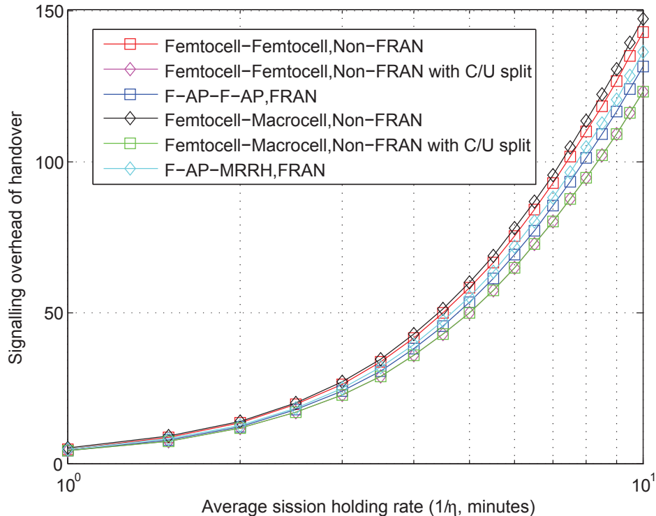
Fig. 5. Signalling overhead versus average session holding rate.
