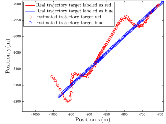
Fig. 7. Estimated position of the targets by the MM filter
