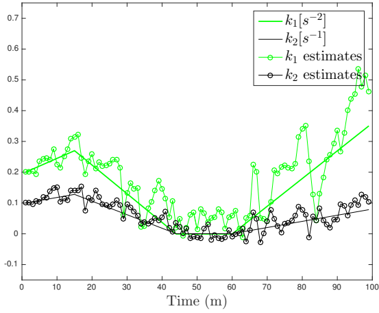
Fig. 9. Estimation of the parameters in the interacting motion model.
