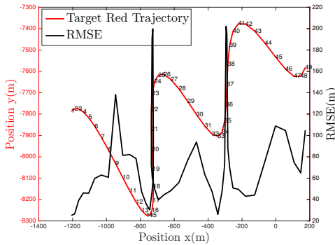
Fig. 3. Error on the position estimates for the target labeled as red by a traditional filter with independent motion assumptions. Estimation error is presented in the same x position axis as the trajectory to show that the maximums in error match the largest accelerations due to targets interaction. Timing information (in seconds) is also provided along the trajectory.
