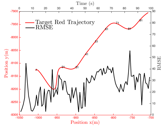
Fig. 12. Error on the position estimates for target labeled as red by a traditional filter with independent motion assumptions.
