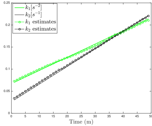
Fig. 6. Estimation of the parameters in the interacting motion model.
