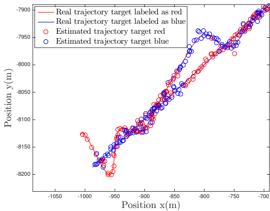
Fig. 11. Position estimates of a traditional filter with independent motion assumptions.
