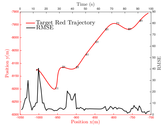
Fig. 8. Error on the position estimates by the MM filter for target labeled as red. Each curve is referenced to the axis scale on its same color. Time scale is also shown over the trajectory.
