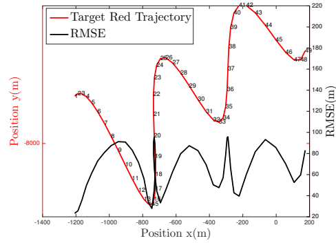
Fig. 5. Error on the position estimates for the target labeled as red by our filter with interacting motion assumptions.
