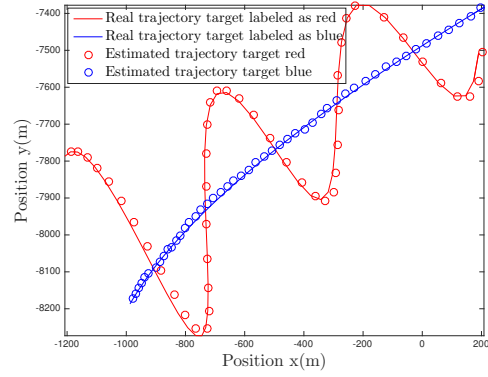
Fig. 4. Position estimates of our filter encapsulating interacting motion assumptions.
