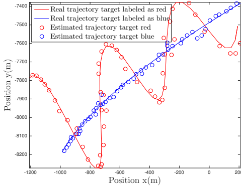
Fig. 2. Position estimates of a traditional filter with independent motion assumptions.
