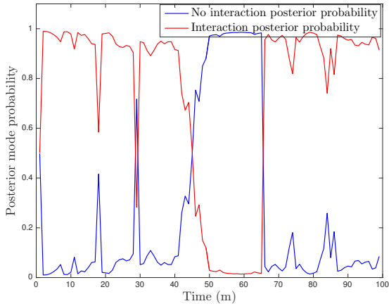
Fig. 10. Estimation of targets behavior
