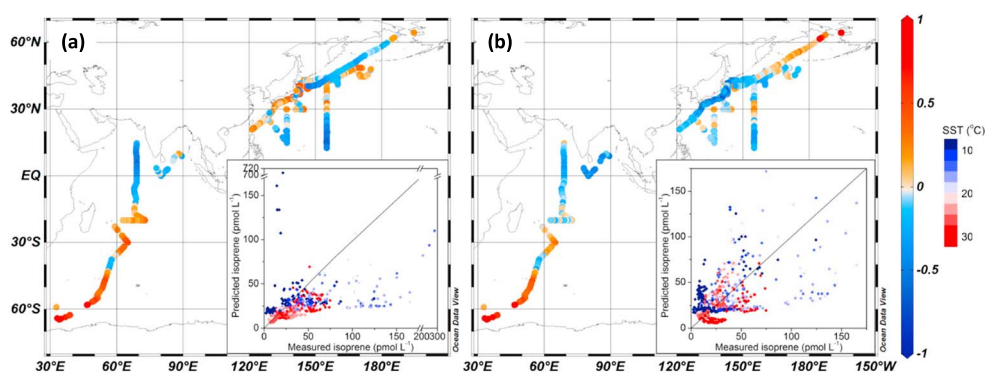
Figure 9. Ratio ( \log_{10} scale) of predicted isoprene from satellite data to the Ooki et al. [2015] data set; (a) using Chl a -based algorithm (one outlier at 1.5) and (b) using intPP-based algorithm (full-scale version of inset graph in supporting information Figure S7). Maps created with Ocean Data View [Schlitzer, 2016].
