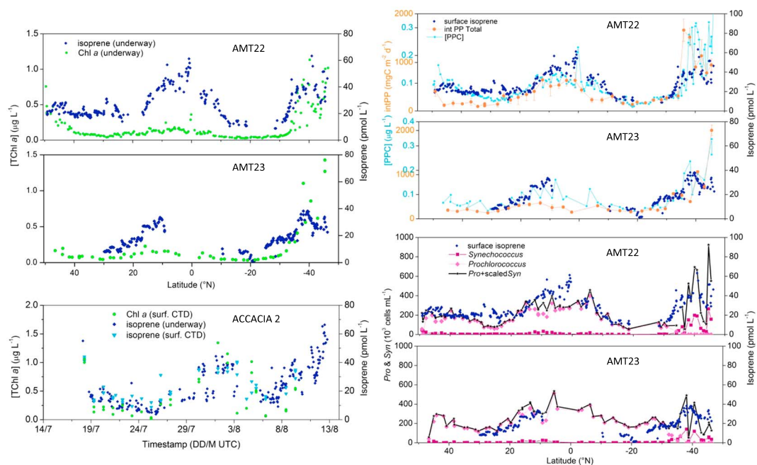
Figure 5. Transect/time series plots of surface ocean isoprene concentrations alongside selected biological measurements: total Chl a , sum of photoprotective carotenoids (PPC); sum of aeaxanthin, alloxanthin, diadinoxanthin, \alpha - and \beta -Carotenes, and diatoxanthin), integrated primary production (intPP total), and Synechococcus and Prochlorococcus cell counts ( Syn , Pro ; Syn in Syn + Pro are scaled by a factor of 3.5 to account for cell-normalized isoprene production rates given in Shaw et al. [2003]).
