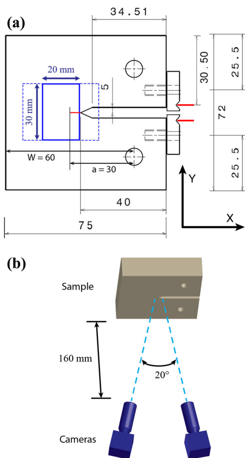
Fig. 2 The experiment geometry: (a) CT specimen dimensions and clip-gauge position, the dotted box shows the area viewed only by one of the two cameras of the set-up, and the smaller solid box represents the calibrated area that was in common between the two cameras; the specimen thickness is 20 mm (b) schematic of the experimental set-up with a 20° angle between the two cameras
