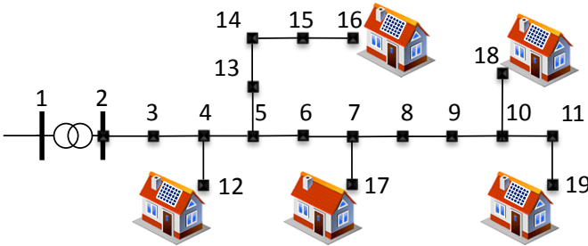
Fig. 1. Cigre LV grid - modified [15].
