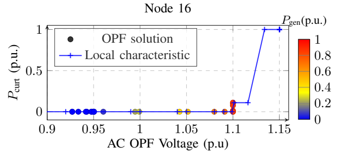
(a) Q = f(V, P) characteristic curve at Node 16.
